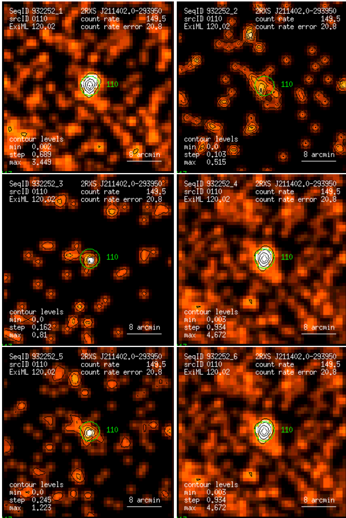
Figure 110: RASS 932252: detection 0110: band rate images, Gaussian filter: (1) PSPC channels 11 – 41, (2) 52 – 90, (3) 91 – 201, (4) 11 – 235, (5) 52 – 201, (6) 11 – 201. Broad band rates in counts/ks. Band rate contour levels in counts/ks/arcmin 2 .
