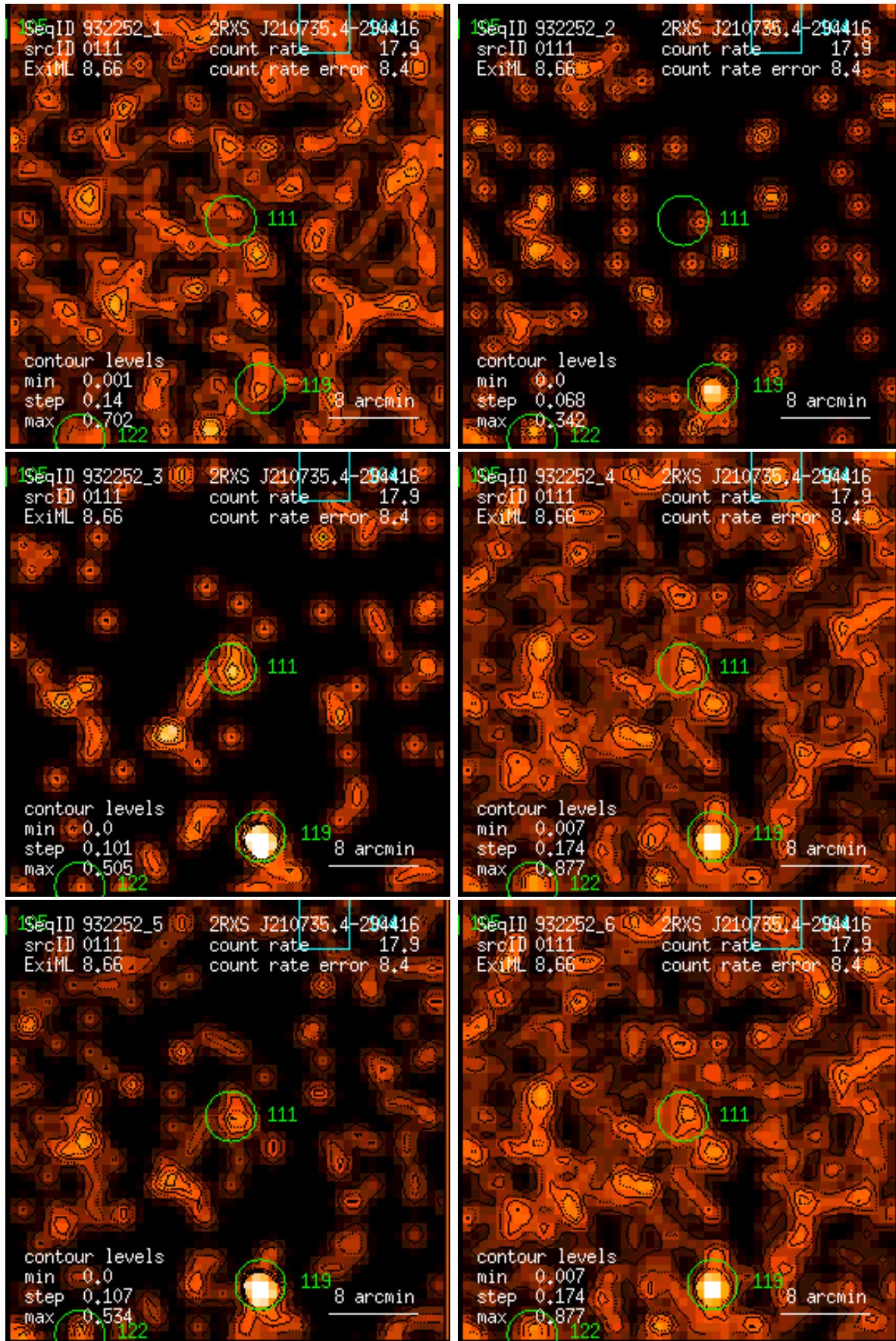
Figure 111: RASS 932252: detection 0111: band rate images, Gaussian filter: (1) PSPC channels 11 – 41, (2) 52 – 90, (3) 91 – 201, (4) 11 – 235, (5) 52 – 201, (6) 11 – 201. Broad band rates in counts/ks. Band rate contour levels in counts/ks/arcmin 2 .
