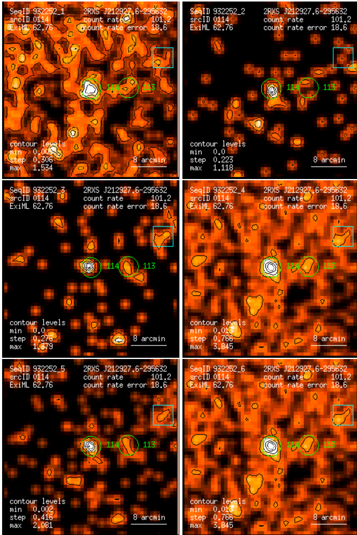
Figure 114: RASS 932252: detection 0114: band rate images, Gaussian filter: (1) PSPC channels 11 – 41, (2) 52 – 90, (3) 91 – 201, (4) 11 – 235, (5) 52 – 201, (6) 11 – 201. Broad band rates in counts/ks. Band rate contour levels in counts/ks/arcmin 2 .
