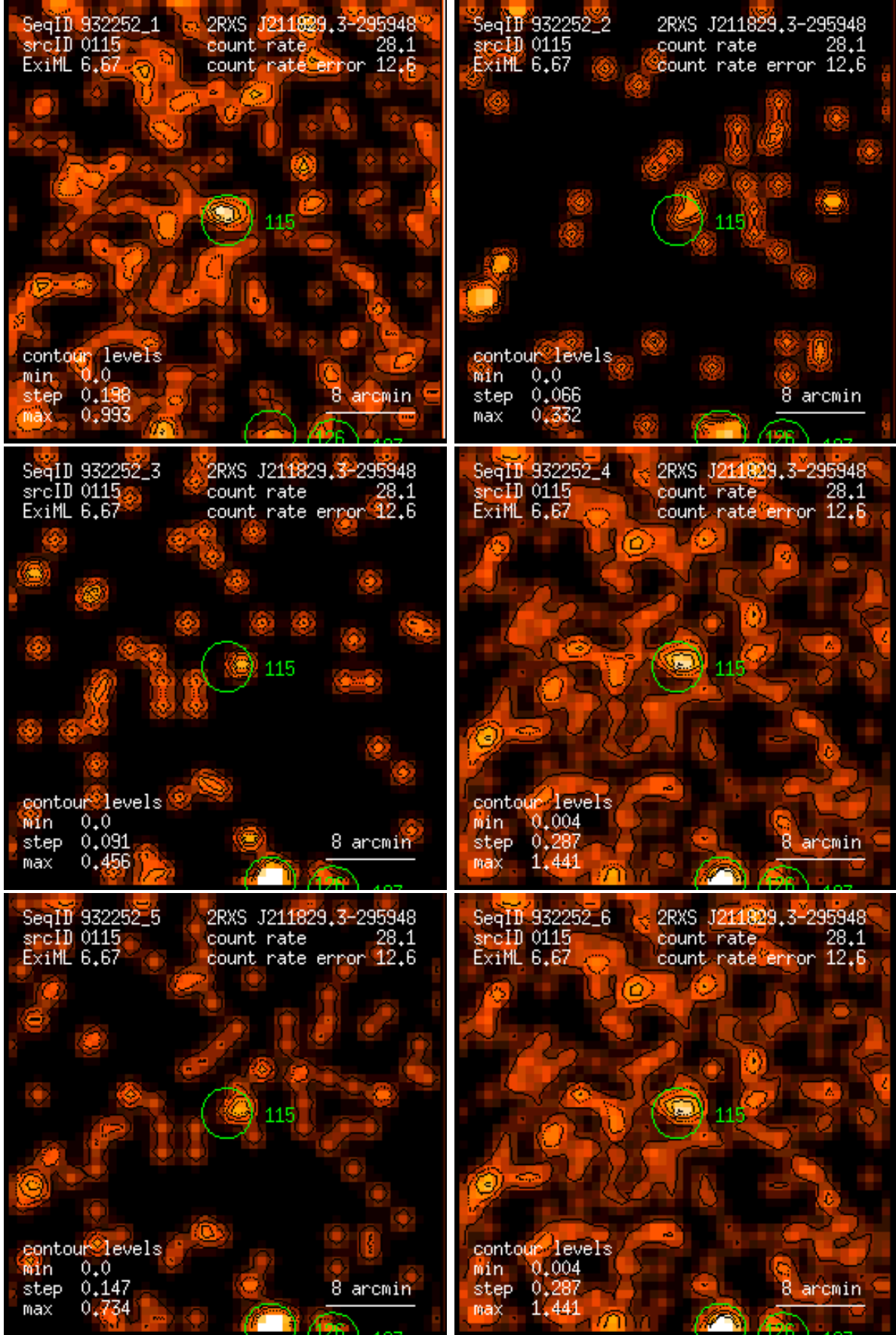
Figure 115: RASS 932252: detection 0115: band rate images, Gaussian filter: (1) PSPC channels 11 – 41, (2) 52 – 90, (3) 91 – 201, (4) 11 – 235, (5) 52 – 201, (6) 11 – 201. Broad band rates in counts/ks. Band rate contour levels in counts/ks/arcmin 2 .
