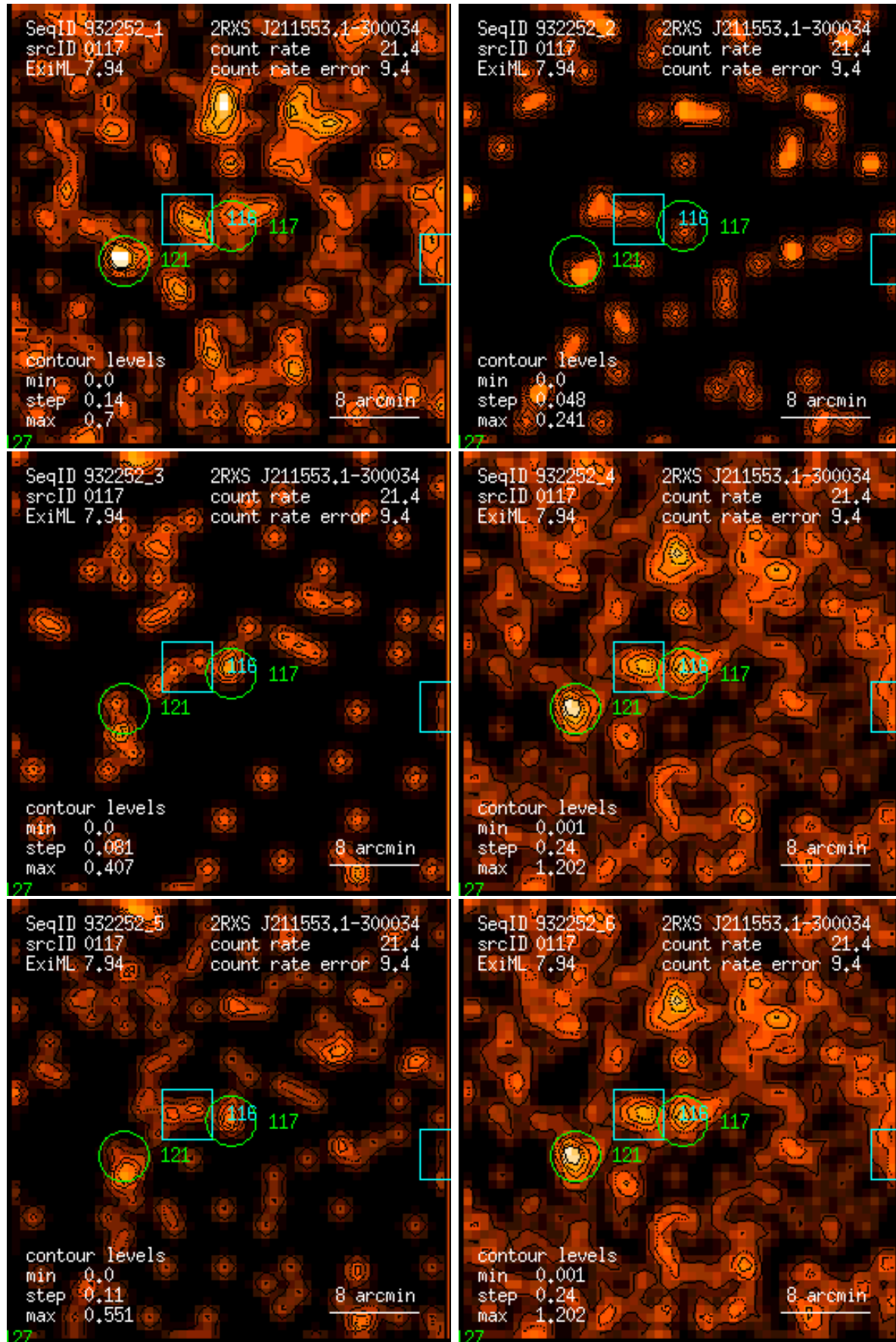
Figure 117: RASS 932252: detection 0117: band rate images, Gaussian filter: (1) PSPC channels 11 – 41, (2) 52 – 90, (3) 91 – 201, (4) 11 – 235, (5) 52 – 201, (6) 11 – 201. Broad band rates in counts/ks. Band rate contour levels in counts/ks/arcmin 2 .
