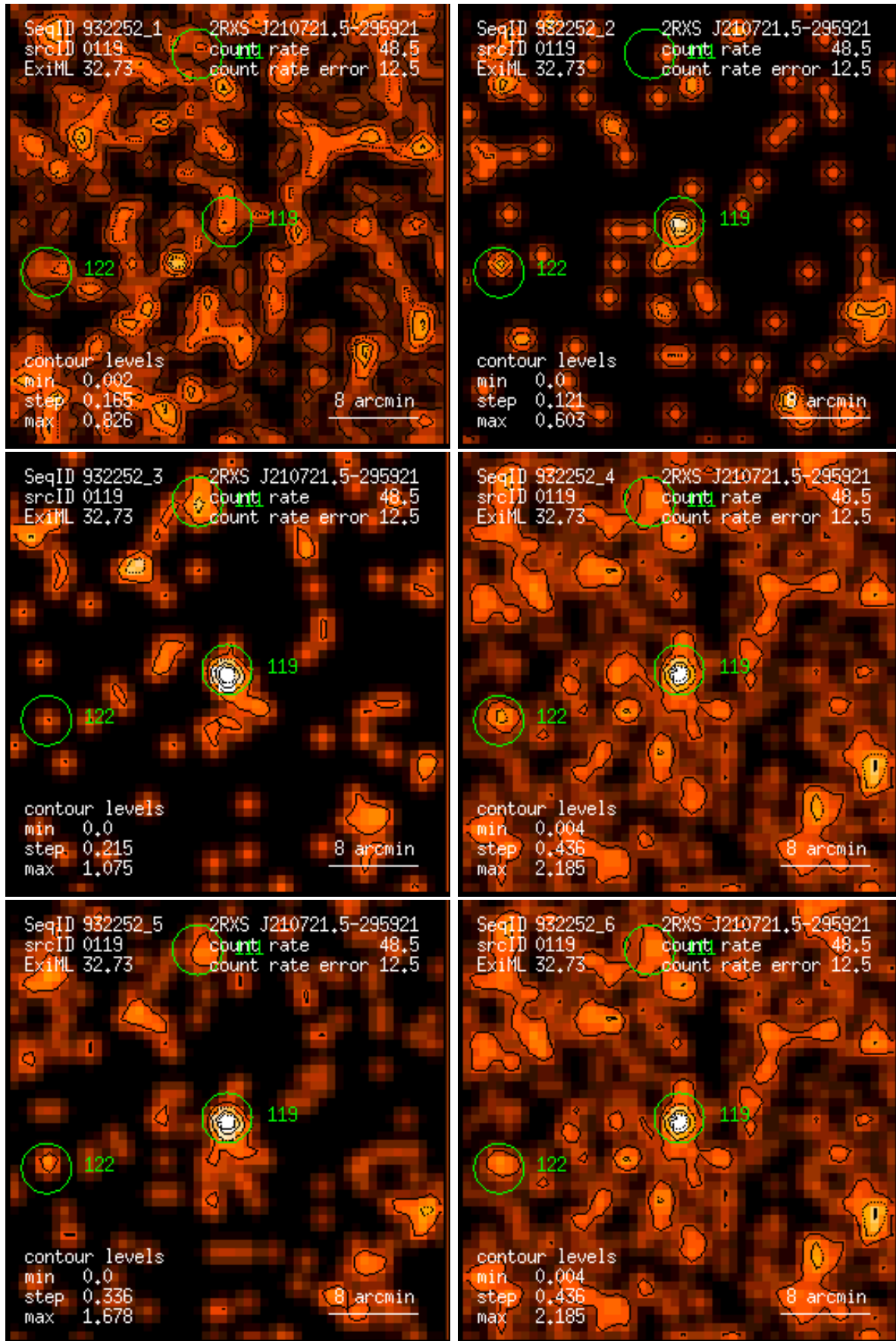
Figure 119: RASS 932252: detection 0119: band rate images, Gaussian filter: (1) PSPC channels 11 – 41, (2) 52 – 90, (3) 91 – 201, (4) 11 – 235, (5) 52 – 201, (6) 11 – 201. Broad band rates in counts/ks. Band rate contour levels in counts/ks/arcmin 2 .
