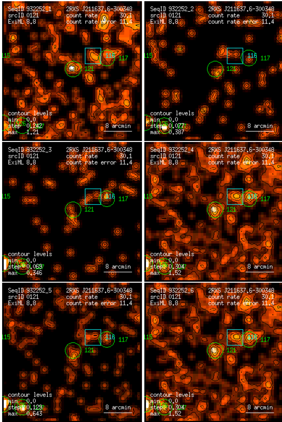
Figure 121: RASS 932252: detection 0121: band rate images, Gaussian filter: (1) PSPC channels 11 – 41, (2) 52 – 90, (3) 91 – 201, (4) 11 – 235, (5) 52 – 201, (6) 11 – 201. Broad band rates in counts/ks. Band rate contour levels in counts/ks/arcmin 2 .
