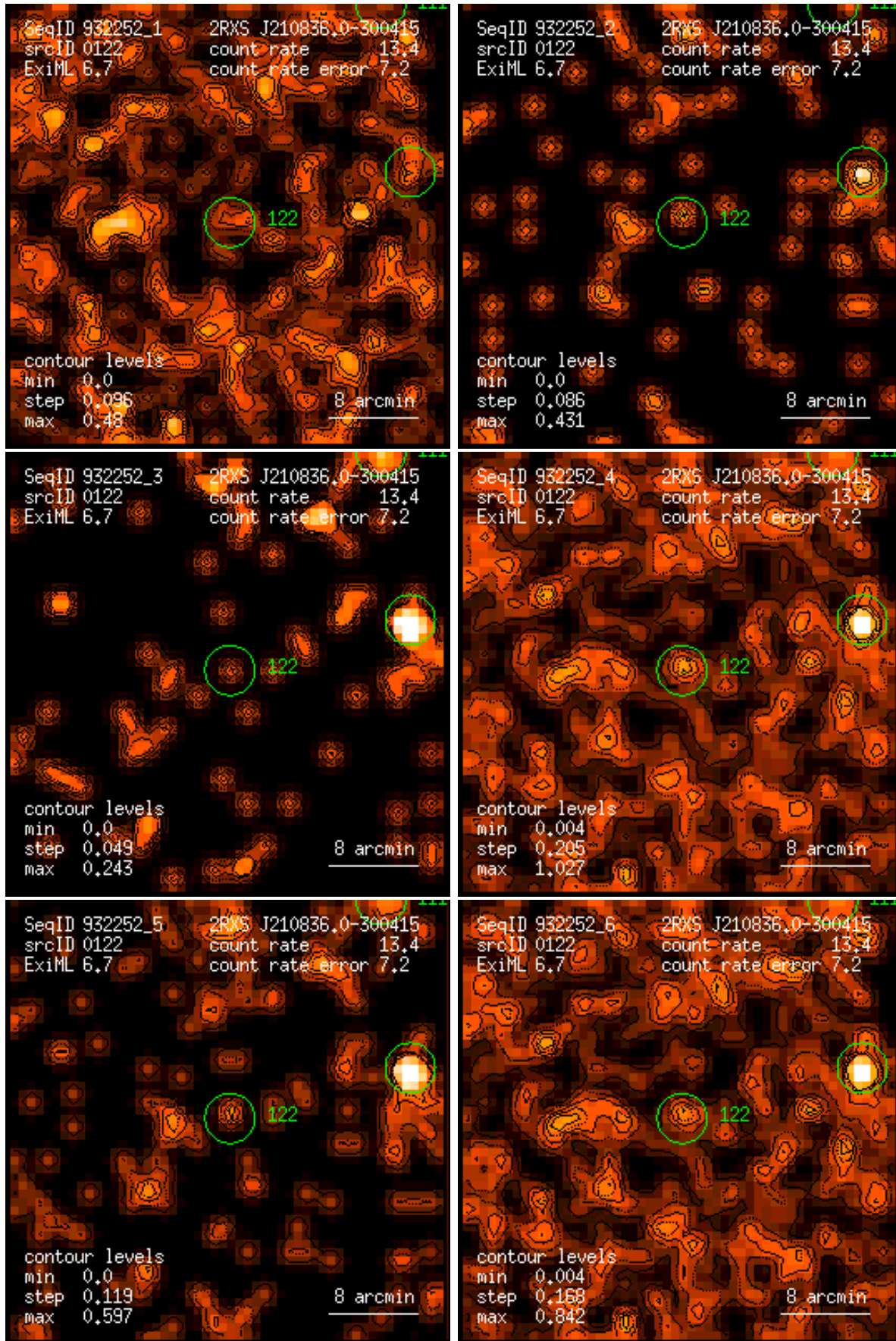
Figure 122: RASS 932252: detection 0122: band rate images, Gaussian filter: (1) PSPC channels 11 – 41, (2) 52 – 90, (3) 91 – 201, (4) 11 – 235, (5) 52 – 201, (6) 11 – 201. Broad band rates in counts/ks. Band rate contour levels in counts/ks/arcmin 2 .
