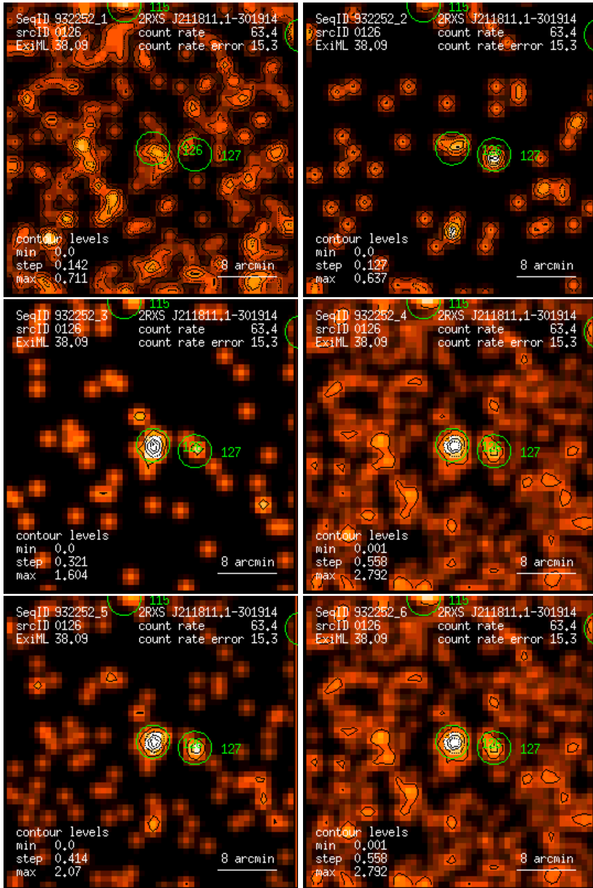
Figure 126: RASS 932252: detection 0126: band rate images, Gaussian filter: (1) PSPC channels 11 – 41, (2) 52 – 90, (3) 91 – 201, (4) 11 – 235, (5) 52 – 201, (6) 11 – 201. Broad band rates in counts/ks. Band rate contour levels in counts/ks/arcmin 2 .
