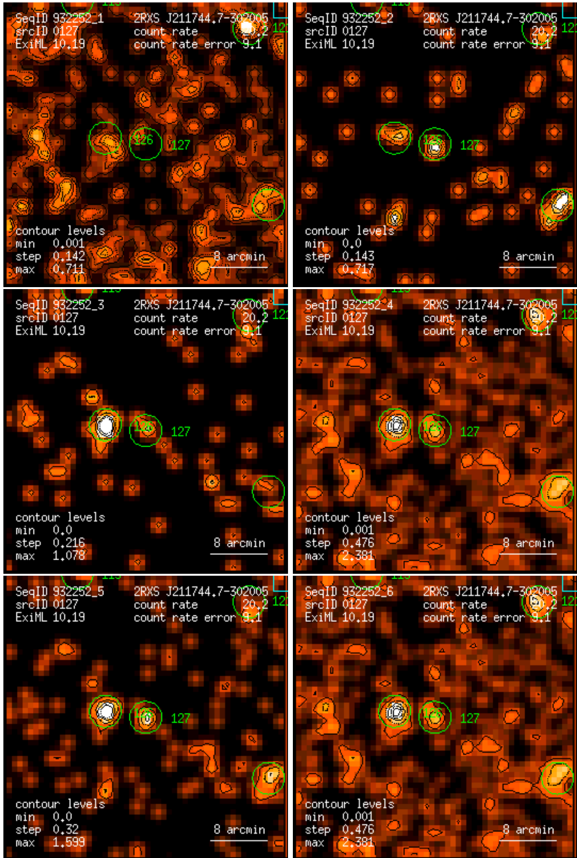
Figure 127: RASS 932252: detection 0127: band rate images, Gaussian filter: (1) PSPC channels 11 – 41, (2) 52 – 90, (3) 91 – 201, (4) 11 – 235, (5) 52 – 201, (6) 11 – 201. Broad band rates in counts/ks. Band rate contour levels in counts/ks/arcmin 2 .
