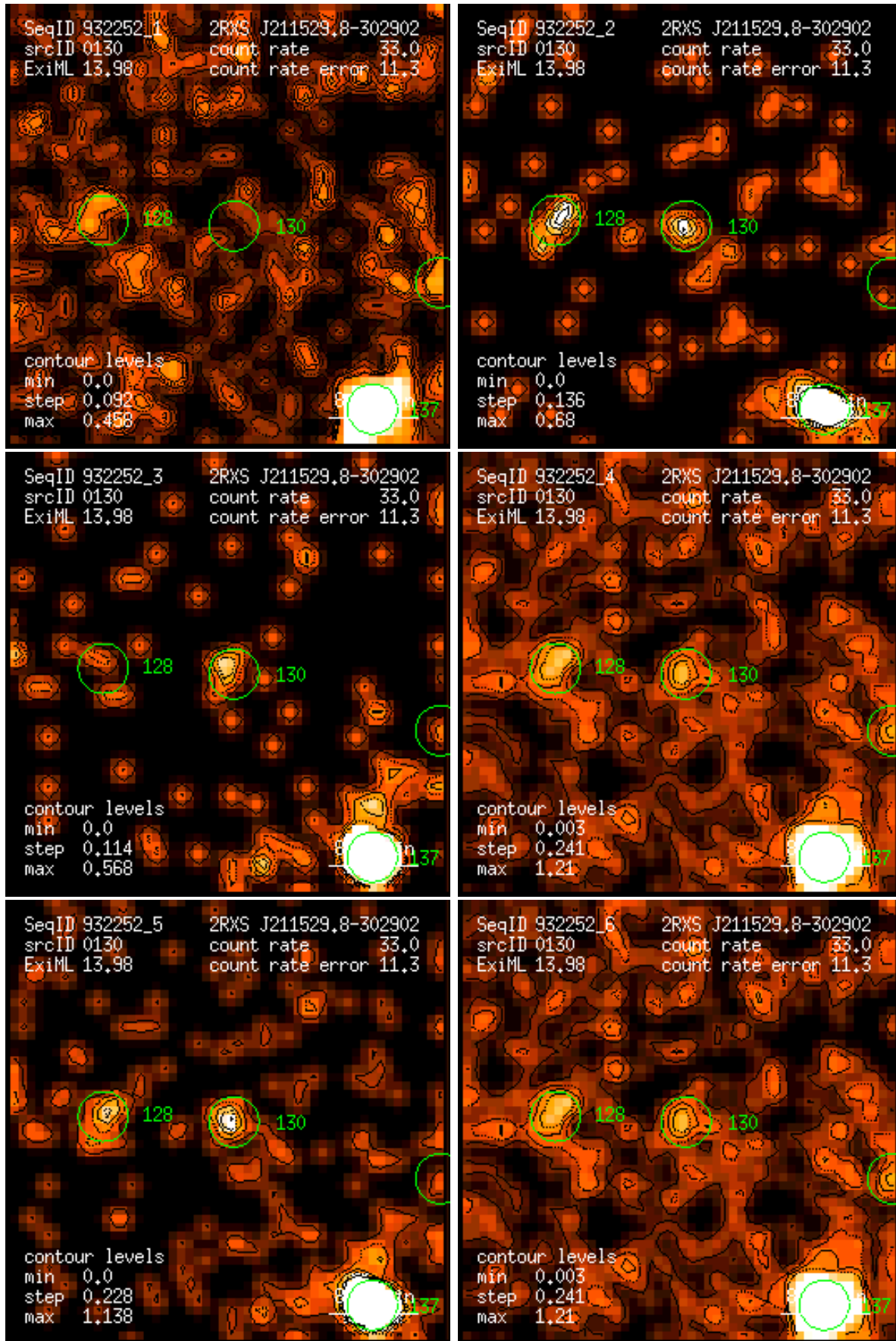
Figure 130: RASS 932252: detection 0130: band rate images, Gaussian filter: (1) PSPC channels 11 – 41, (2) 52 – 90, (3) 91 – 201, (4) 11 – 235, (5) 52 – 201, (6) 11 – 201. Broad band rates in counts/ks. Band rate contour levels in counts/ks/arcmin 2 .
