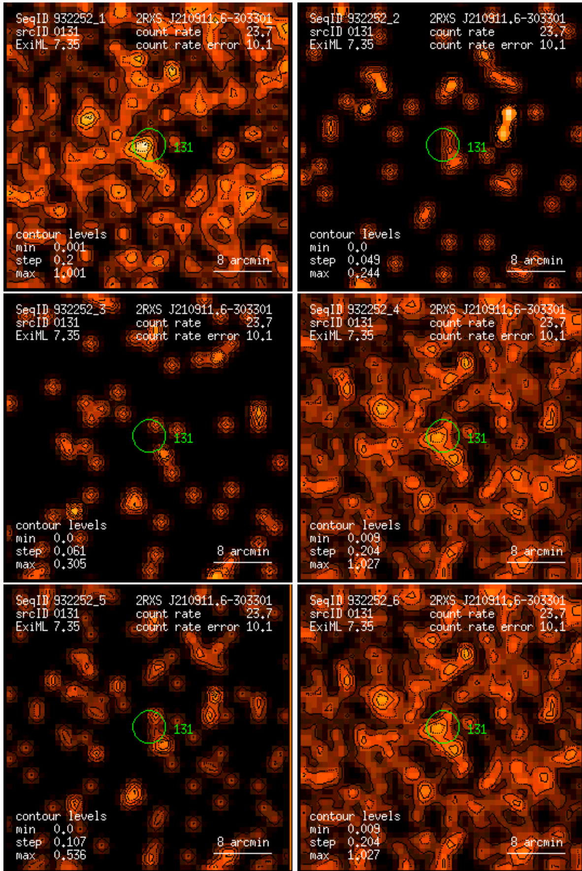
Figure 131: RASS 932252: detection 0131: band rate images, Gaussian filter: (1) PSPC channels 11 – 41, (2) 52 – 90, (3) 91 – 201, (4) 11 – 235, (5) 52 – 201, (6) 11 – 201. Broad band rates in counts/ks. Band rate contour levels in counts/ks/arcmin 2 .
