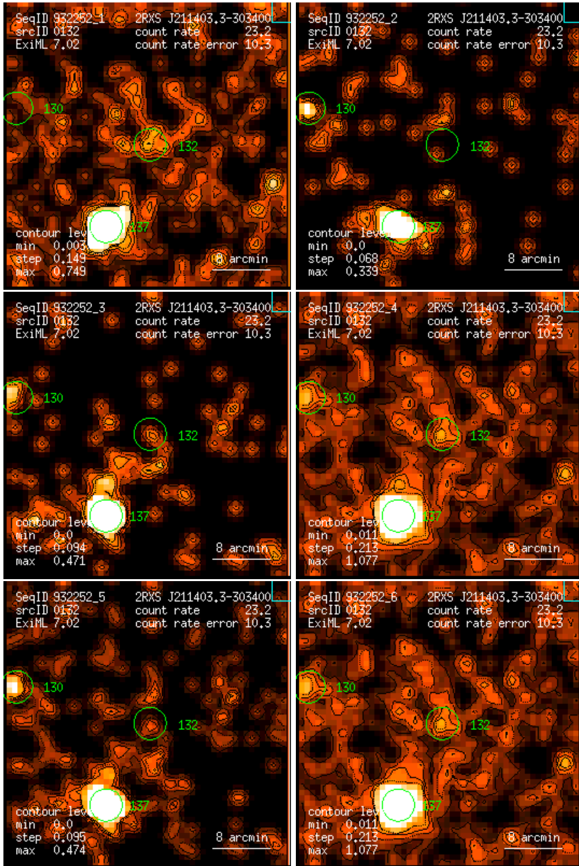
Figure 132: RASS 932252: detection 0132: band rate images, Gaussian filter: (1) PSPC channels 11 – 41, (2) 52 – 90, (3) 91 – 201, (4) 11 – 235, (5) 52 – 201, (6) 11 – 201. Broad band rates in counts/ks. Band rate contour levels in counts/ks/arcmin 2 .
