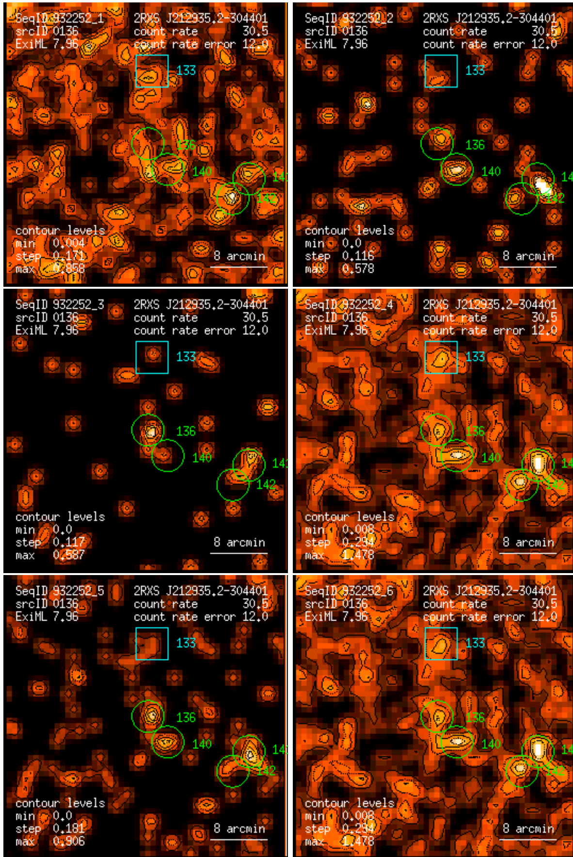
Figure 136: RASS 932252: detection 0136: band rate images, Gaussian filter: (1) PSPC channels 11 – 41, (2) 52 – 90, (3) 91 – 201, (4) 11 – 235, (5) 52 – 201, (6) 11 – 201. Broad band rates in counts/ks. Band rate contour levels in counts/ks/arcmin 2 .
