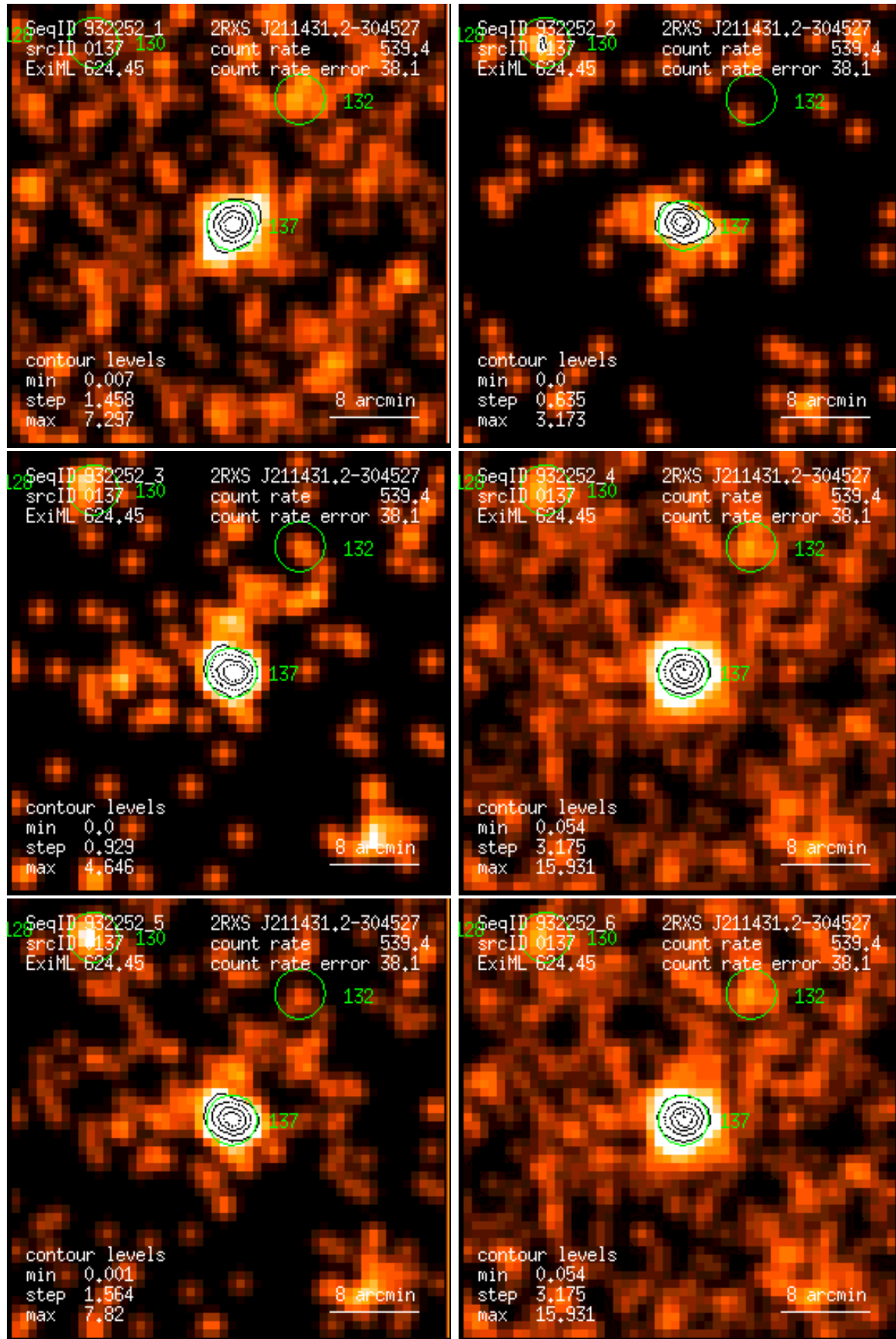
Figure 137: RASS 932252: detection 0137: band rate images, Gaussian filter: (1) PSPC channels 11 – 41, (2) 52 – 90, (3) 91 – 201, (4) 11 – 235, (5) 52 – 201, (6) 11 – 201. Broad band rates in counts/ks. Band rate contour levels in counts/ks/arcmin 2 .
