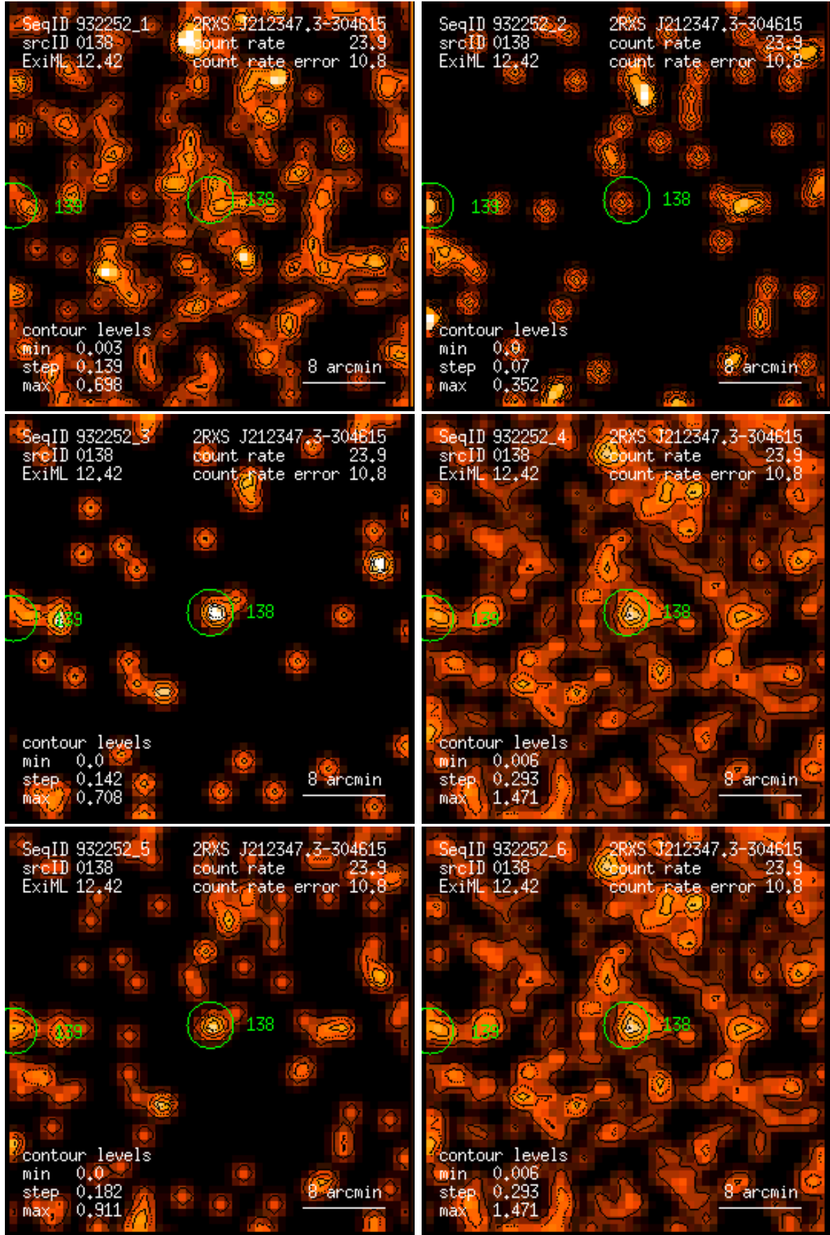
Figure 138: RASS 932252: detection 0138: band rate images, Gaussian filter: (1) PSPC channels 11 – 41, (2) 52 – 90, (3) 91 – 201, (4) 11 – 235, (5) 52 – 201, (6) 11 – 201. Broad band rates in counts/ks. Band rate contour levels in counts/ks/arcmin 2 .
