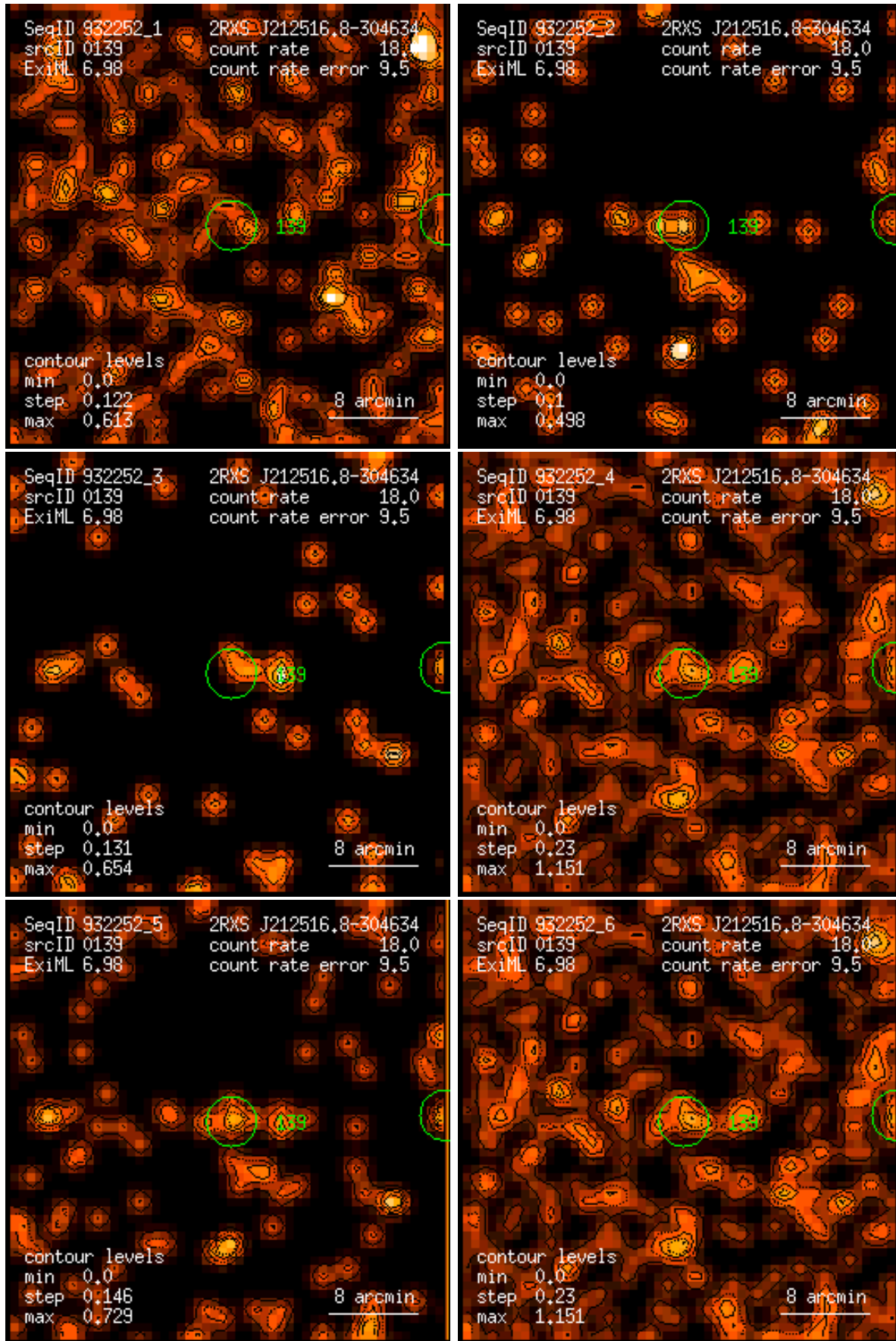
Figure 139: RASS 932252: detection 0139: band rate images, Gaussian filter: (1) PSPC channels 11 – 41, (2) 52 – 90, (3) 91 – 201, (4) 11 – 235, (5) 52 – 201, (6) 11 – 201. Broad band rates in counts/ks. Band rate contour levels in counts/ks/arcmin 2 .
