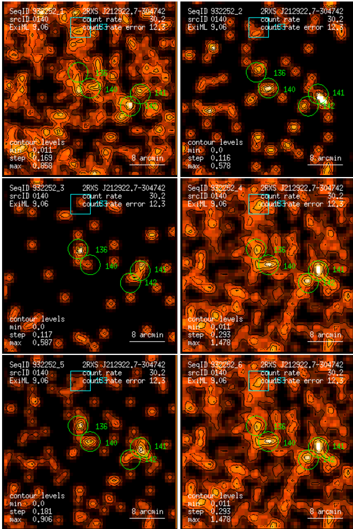
Figure 140: RASS 932252: detection 0140: band rate images, Gaussian filter: (1) PSPC channels 11 – 41, (2) 52 – 90, (3) 91 – 201, (4) 11 – 235, (5) 52 – 201, (6) 11 – 201. Broad band rates in counts/ks. Band rate contour levels in counts/ks/arcmin 2 .
