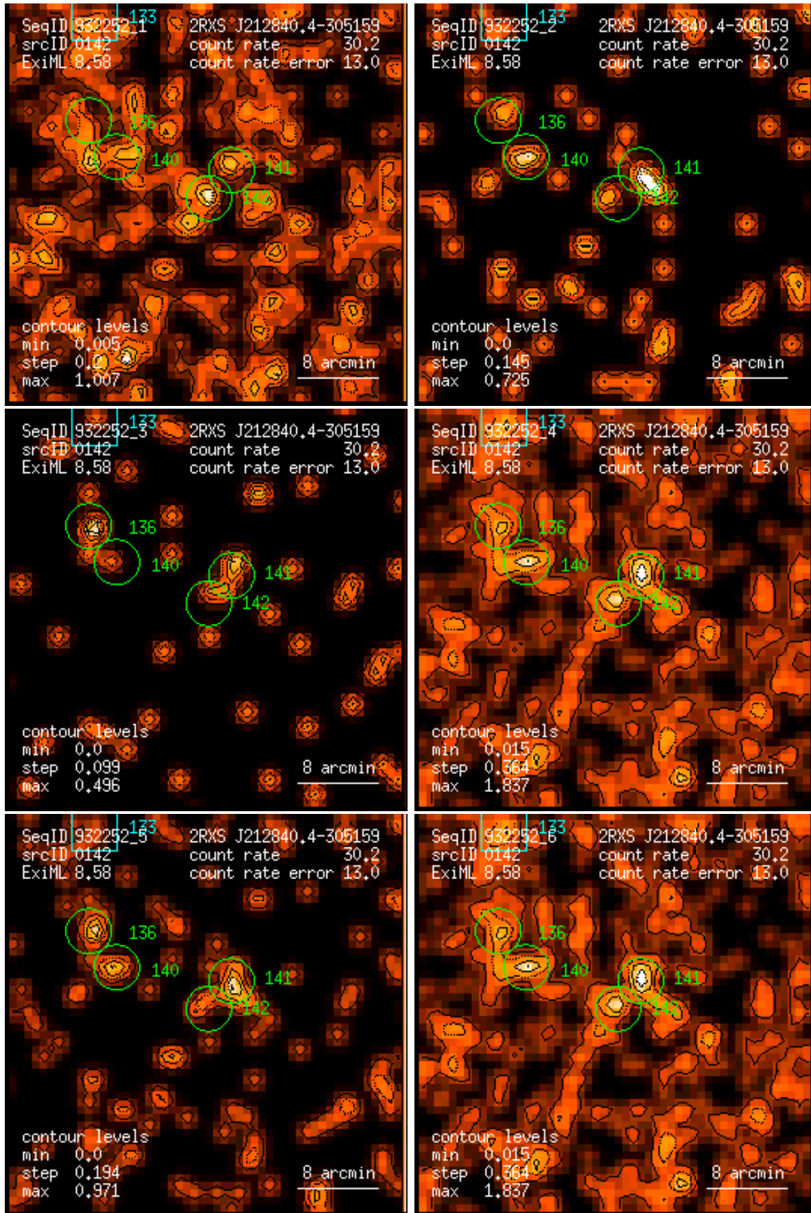
Figure 142: RASS 932252: detection 0142: band rate images, Gaussian filter: (1) PSPC channels 11 – 41, (2) 52 – 90, (3) 91 – 201, (4) 11 – 235, (5) 52 – 201, (6) 11 – 201. Broad band rates in counts/ks. Band rate contour levels in counts/ks/arcmin 2 .
