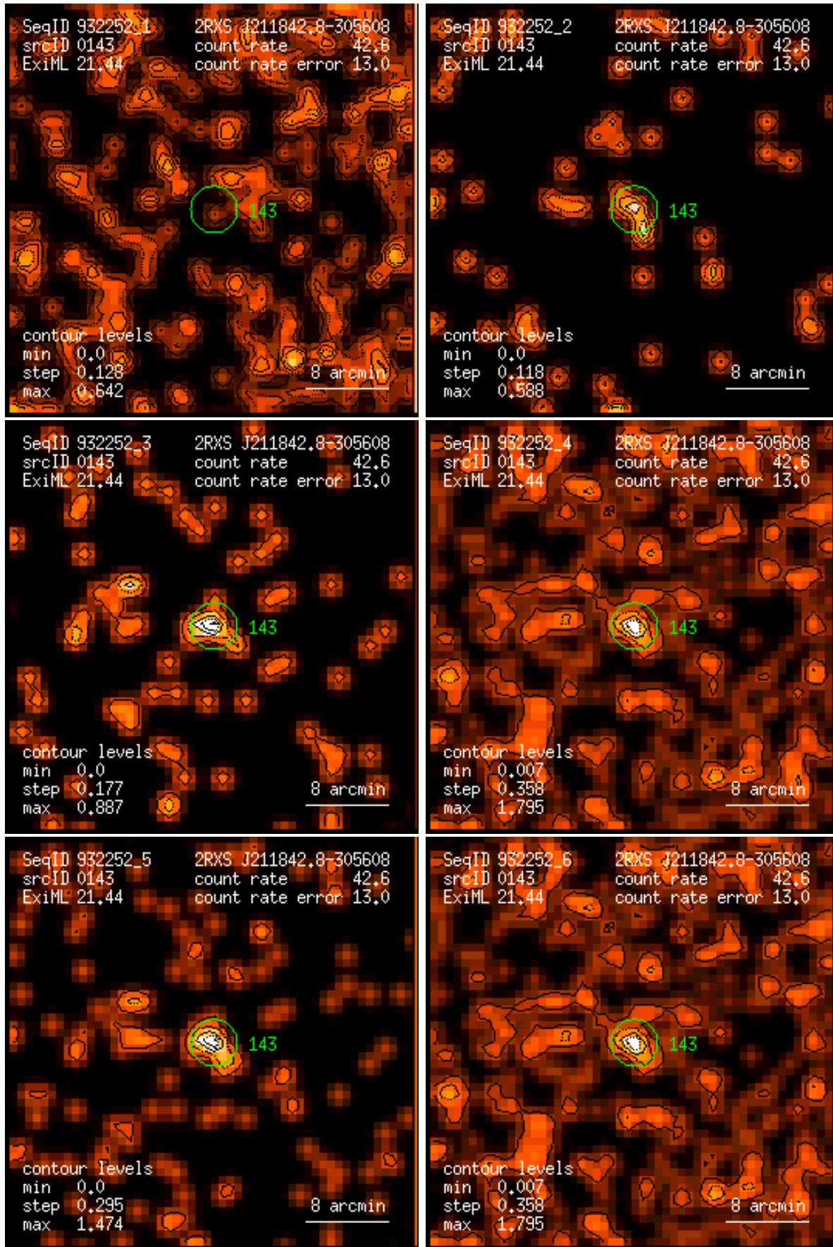
Figure 143: RASS 932252: detection 0143: band rate images, Gaussian filter: (1) PSPC channels 11 – 41, (2) 52 – 90, (3) 91 – 201, (4) 11 – 235, (5) 52 – 201, (6) 11 – 201. Broad band rates in counts/ks. Band rate contour levels in counts/ks/arcmin 2 .
