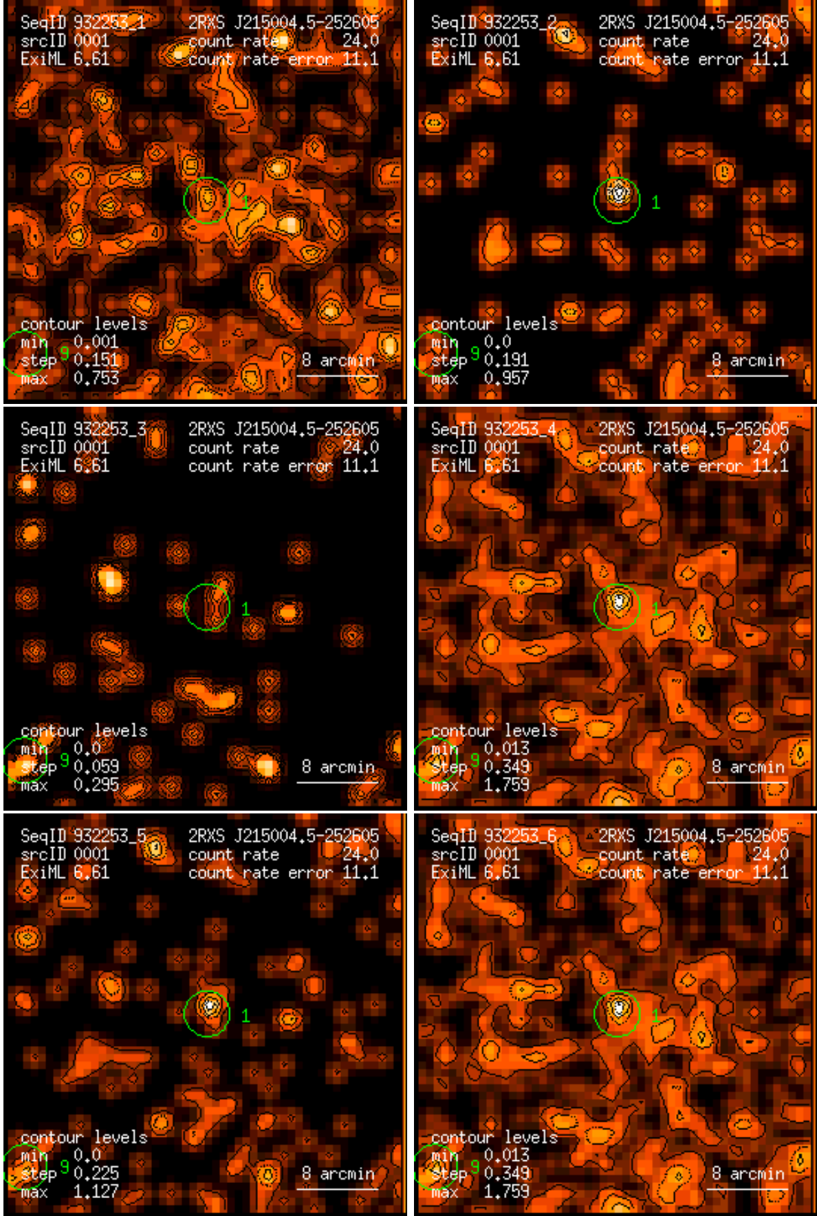
Figure 1: RASS 932253: detection 0001: band rate images, Gaussian filter: (1) PSPC channels 11 – 41, (2) 52 – 90, (3) 91 – 201, (4) 11 – 235, (5) 52 – 201, (6) 11 – 201. Broad band rates in counts/ks. Band rate contour levels in counts/ks/arcmin 2 .
