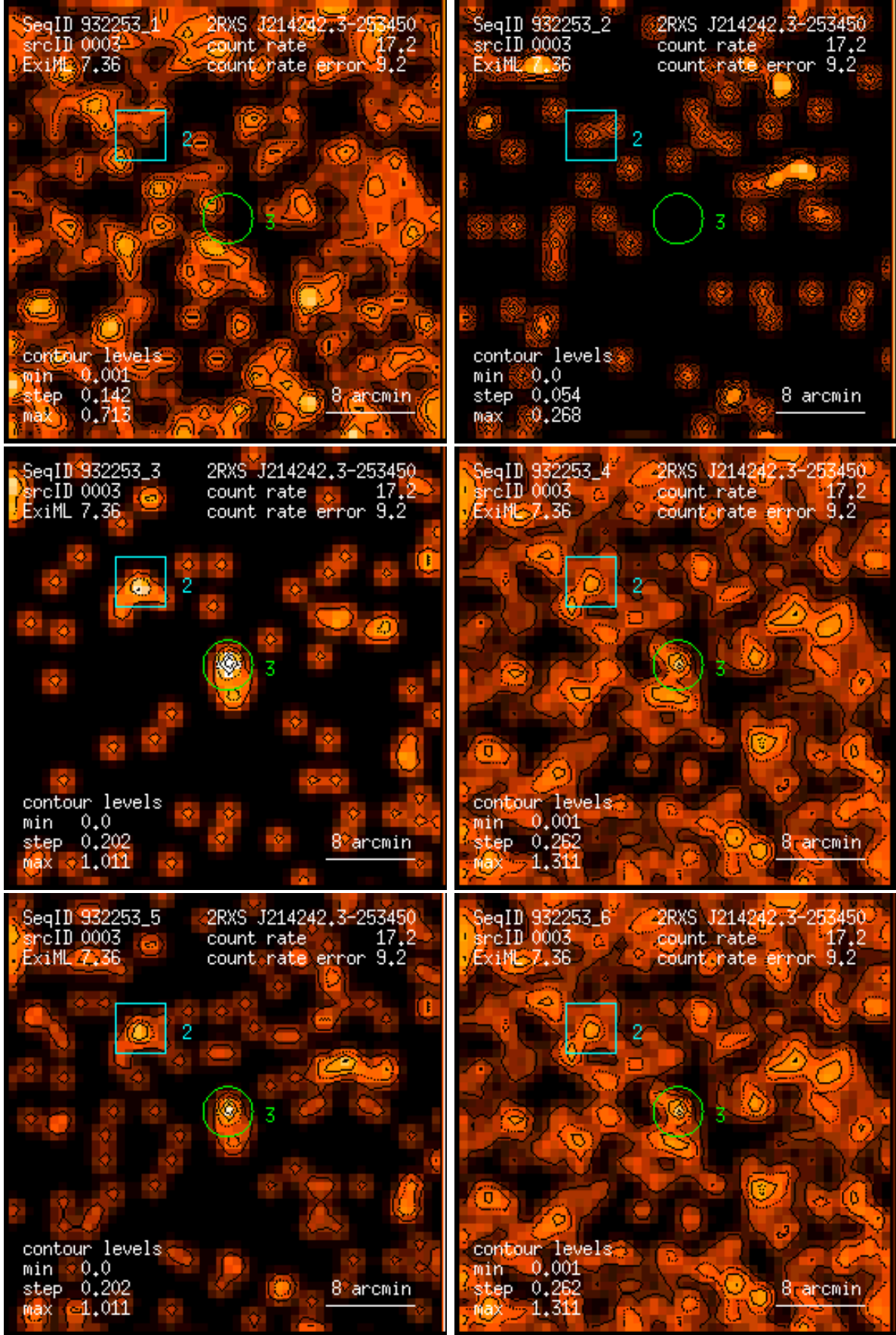
Figure 3: RASS 932253: detection 0003: band rate images, Gaussian filter: (1) PSPC channels 11 – 41, (2) 52 – 90, (3) 91 – 201, (4) 11 – 235, (5) 52 – 201, (6) 11 – 201. Broad band rates in counts/ks. Band rate contour levels in counts/ks/arcmin 2 .
