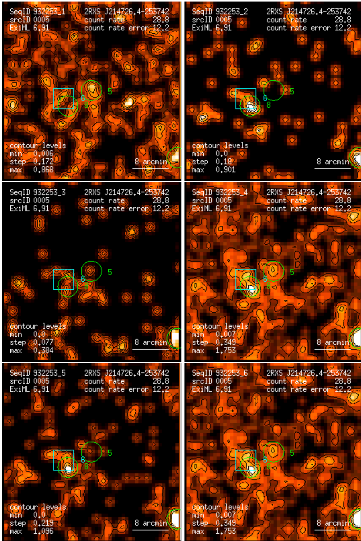
Figure 5: RASS 932253: detection 0005: band rate images, Gaussian filter: (1) PSPC channels 11 – 41, (2) 52 – 90, (3) 91 – 201, (4) 11 – 235, (5) 52 – 201, (6) 11 – 201. Broad band rates in counts/ks. Band rate contour levels in counts/ks/arcmin 2 .
