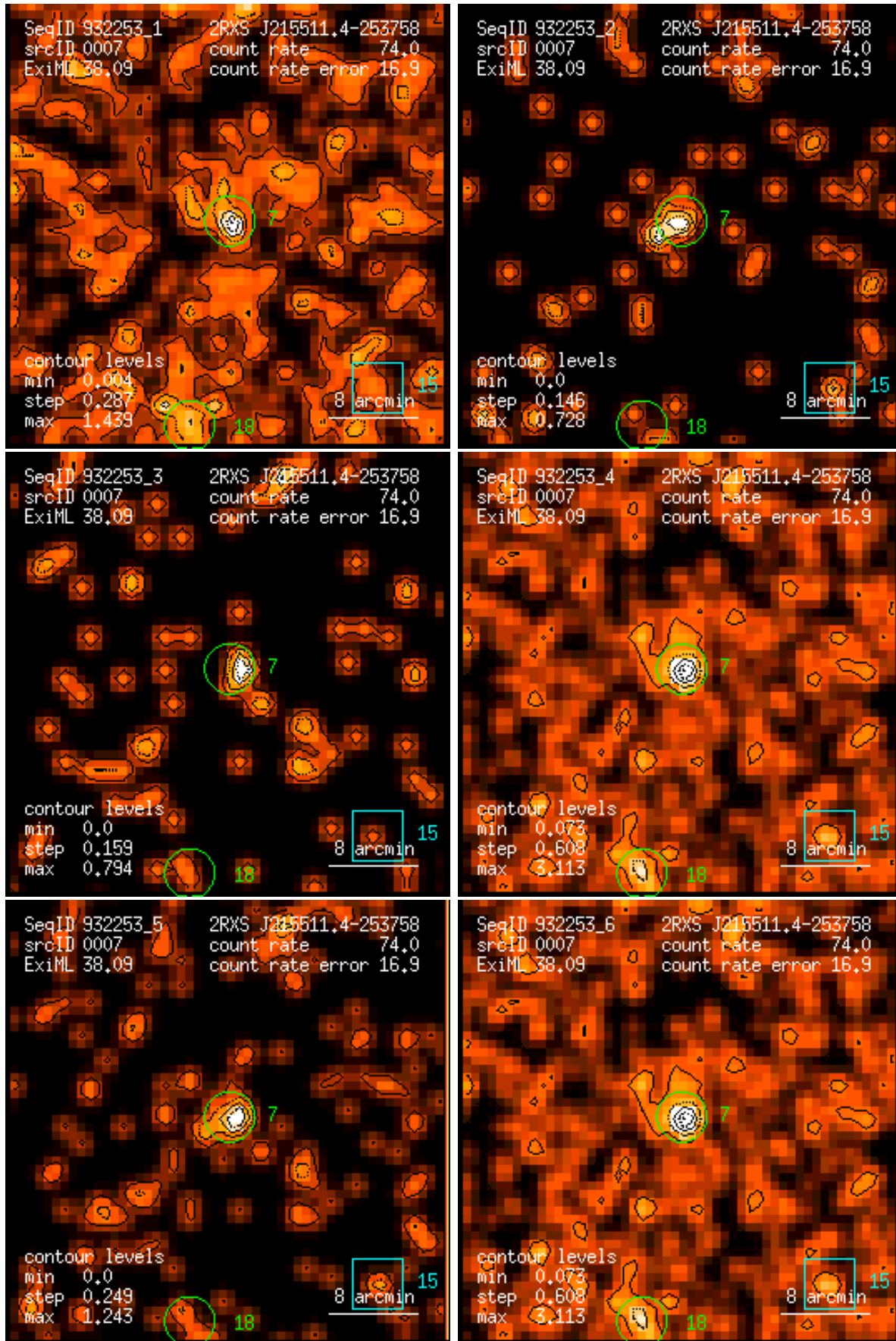
Figure 7: RASS 932253: detection 0007: band rate images, Gaussian filter: (1) PSPC channels 11 – 41, (2) 52 – 90, (3) 91 – 201, (4) 11 – 235, (5) 52 – 201, (6) 11 – 201. Broad band rates in counts/ks. Band rate contour levels in counts/ks/arcmin 2 .
