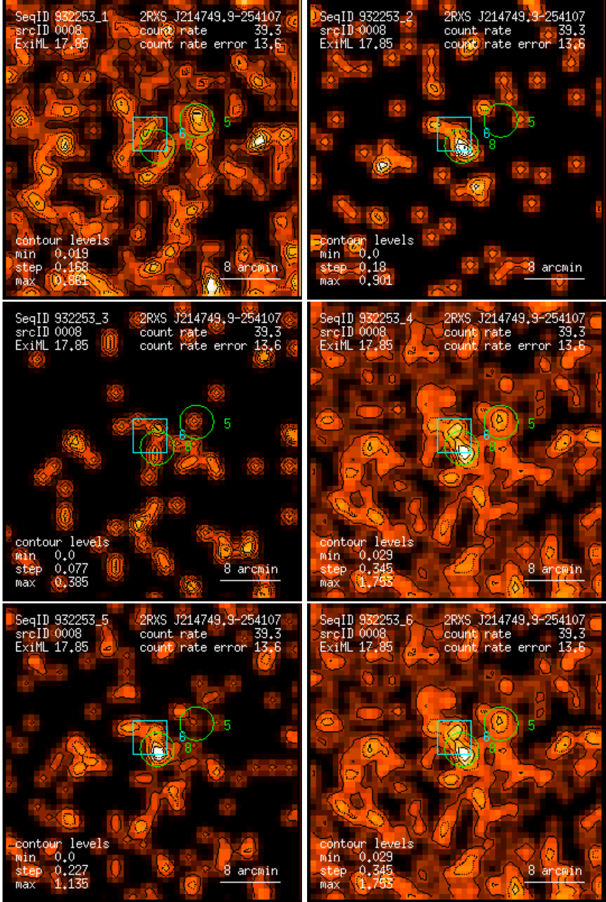
Figure 8: RASS 932253: detection 0008: band rate images, Gaussian filter: (1) PSPC channels 11 – 41, (2) 52 – 90, (3) 91 – 201, (4) 11 – 235, (5) 52 – 201, (6) 11 – 201. Broad band rates in counts/ks. Band rate contour levels in counts/ks/arcmin 2 .
