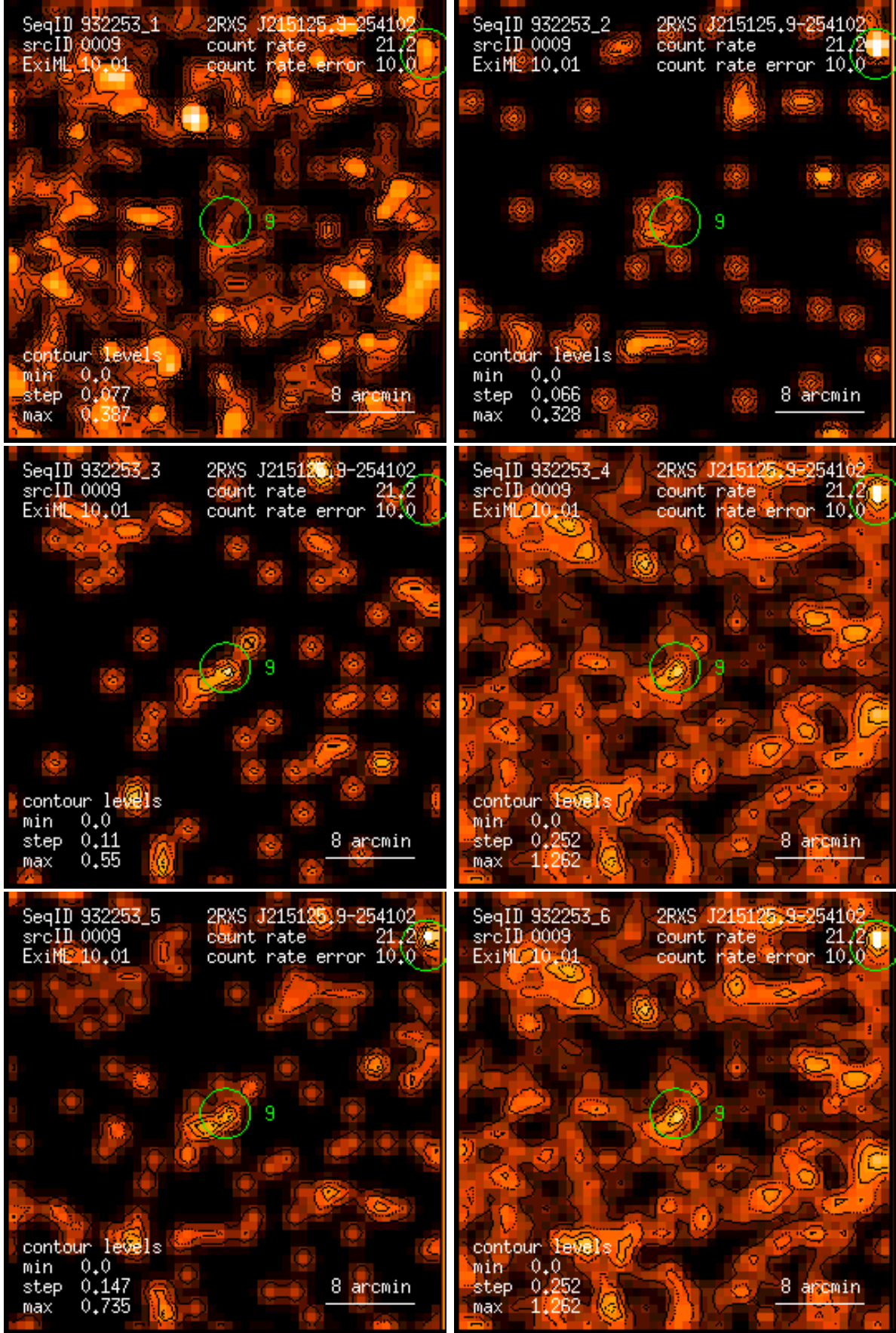
Figure 9: RASS 932253: detection 0009: band rate images, Gaussian filter: (1) PSPC channels 11 – 41, (2) 52 – 90, (3) 91 – 201, (4) 11 – 235, (5) 52 – 201, (6) 11 – 201. Broad band rates in counts/ks. Band rate contour levels in counts/ks/arcmin 2 .
