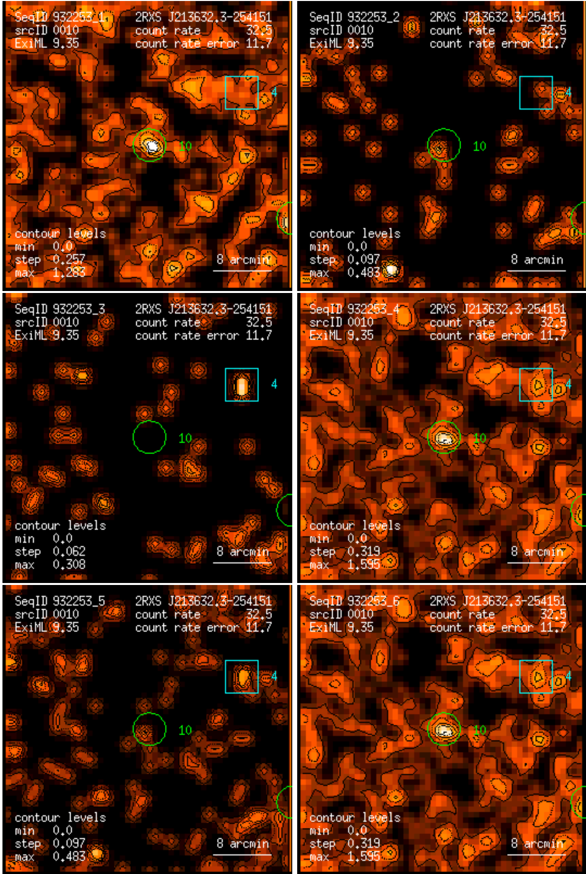
Figure 10: RASS 932253: detection 0010: band rate images, Gaussian filter: (1) PSPC channels 11 – 41, (2) 52 – 90, (3) 91 – 201, (4) 11 – 235, (5) 52 – 201, (6) 11 – 201. Broad band rates in counts/ks. Band rate contour levels in counts/ks/arcmin 2 .
