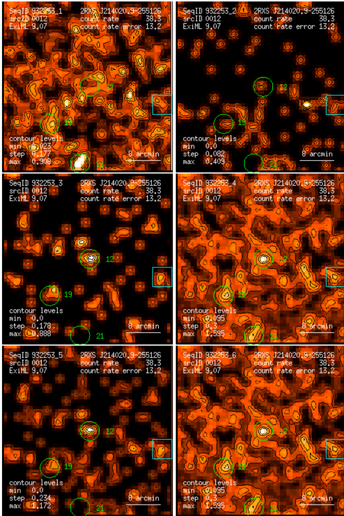
Figure 12: RASS 932253: detection 0012: band rate images, Gaussian filter: (1) PSPC channels 11 – 41, (2) 52 – 90, (3) 91 – 201, (4) 11 – 235, (5) 52 – 201, (6) 11 – 201. Broad band rates in counts/ks. Band rate contour levels in counts/ks/arcmin 2 .
