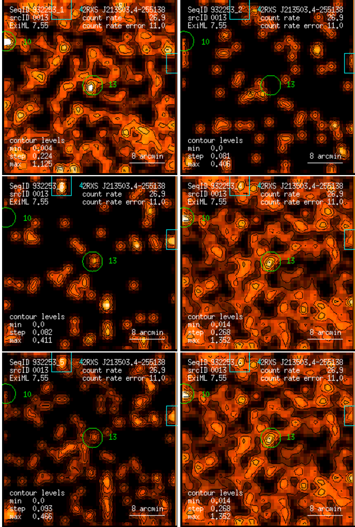
Figure 13: RASS 932253: detection 0013: band rate images, Gaussian filter: (1) PSPC channels 11 – 41, (2) 52 – 90, (3) 91 – 201, (4) 11 – 235, (5) 52 – 201, (6) 11 – 201. Broad band rates in counts/ks. Band rate contour levels in counts/ks/arcmin 2 .
