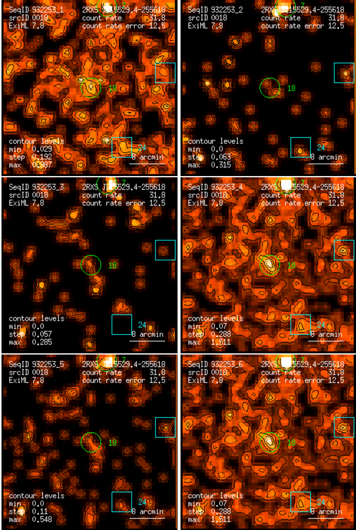
Figure 18: RASS 932253: detection 0018: band rate images, Gaussian filter: (1) PSPC channels 11 – 41, (2) 52 – 90, (3) 91 – 201, (4) 11 – 235, (5) 52 – 201, (6) 11 – 201. Broad band rates in counts/ks. Band rate contour levels in counts/ks/arcmin 2 .
