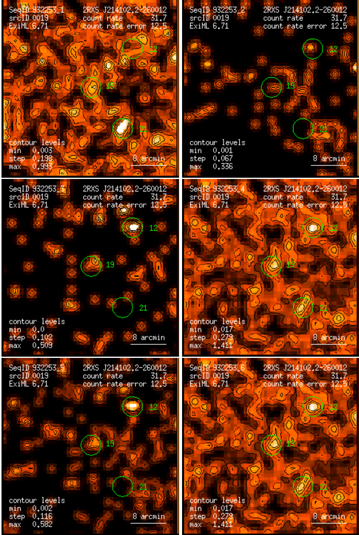
Figure 19: RASS 932253: detection 0019: band rate images, Gaussian filter: (1) PSPC channels 11 – 41, (2) 52 – 90, (3) 91 – 201, (4) 11 – 235, (5) 52 – 201, (6) 11 – 201. Broad band rates in counts/ks. Band rate contour levels in counts/ks/arcmin 2 .
