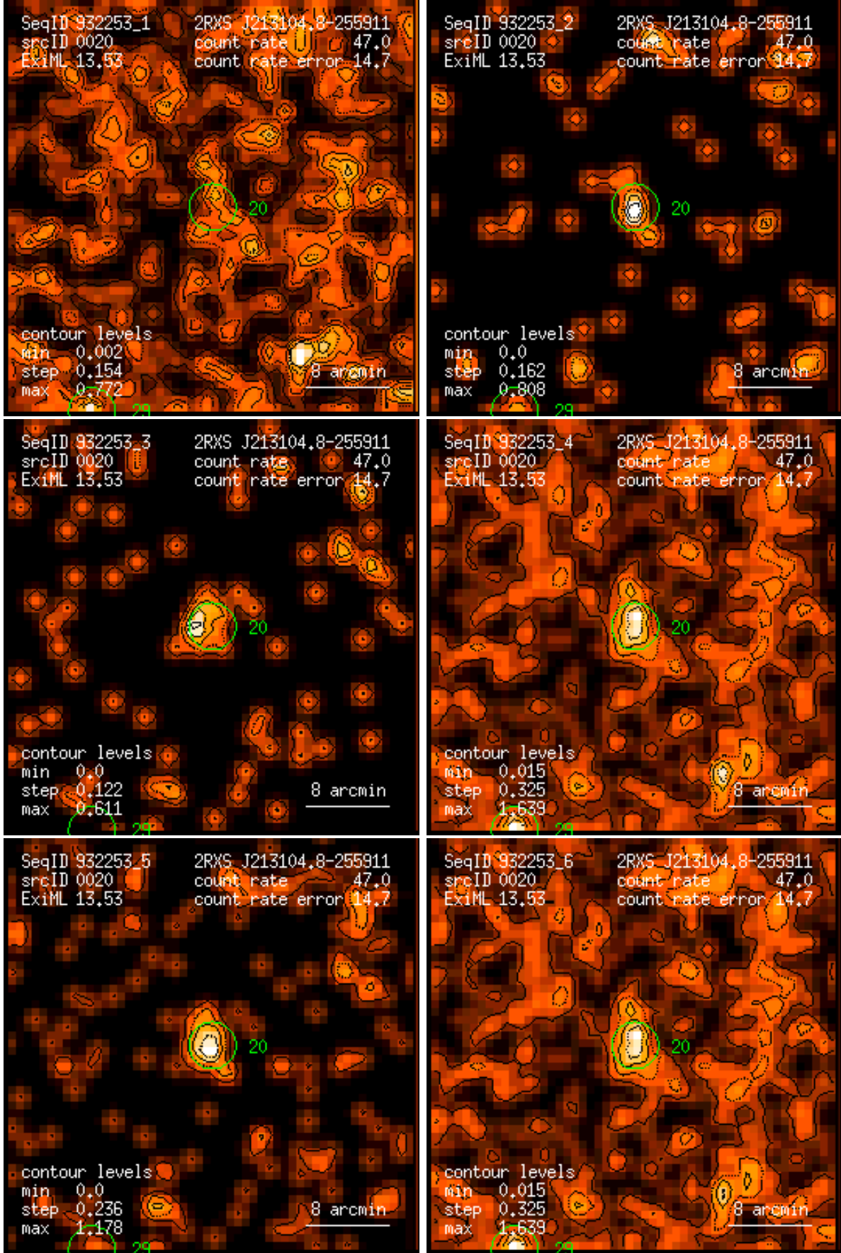
Figure 20: RASS 932253: detection 0020: band rate images, Gaussian filter: (1) PSPC channels 11 – 41, (2) 52 – 90, (3) 91 – 201, (4) 11 – 235, (5) 52 – 201, (6) 11 – 201. Broad band rates in counts/ks. Band rate contour levels in counts/ks/arcmin 2 .
