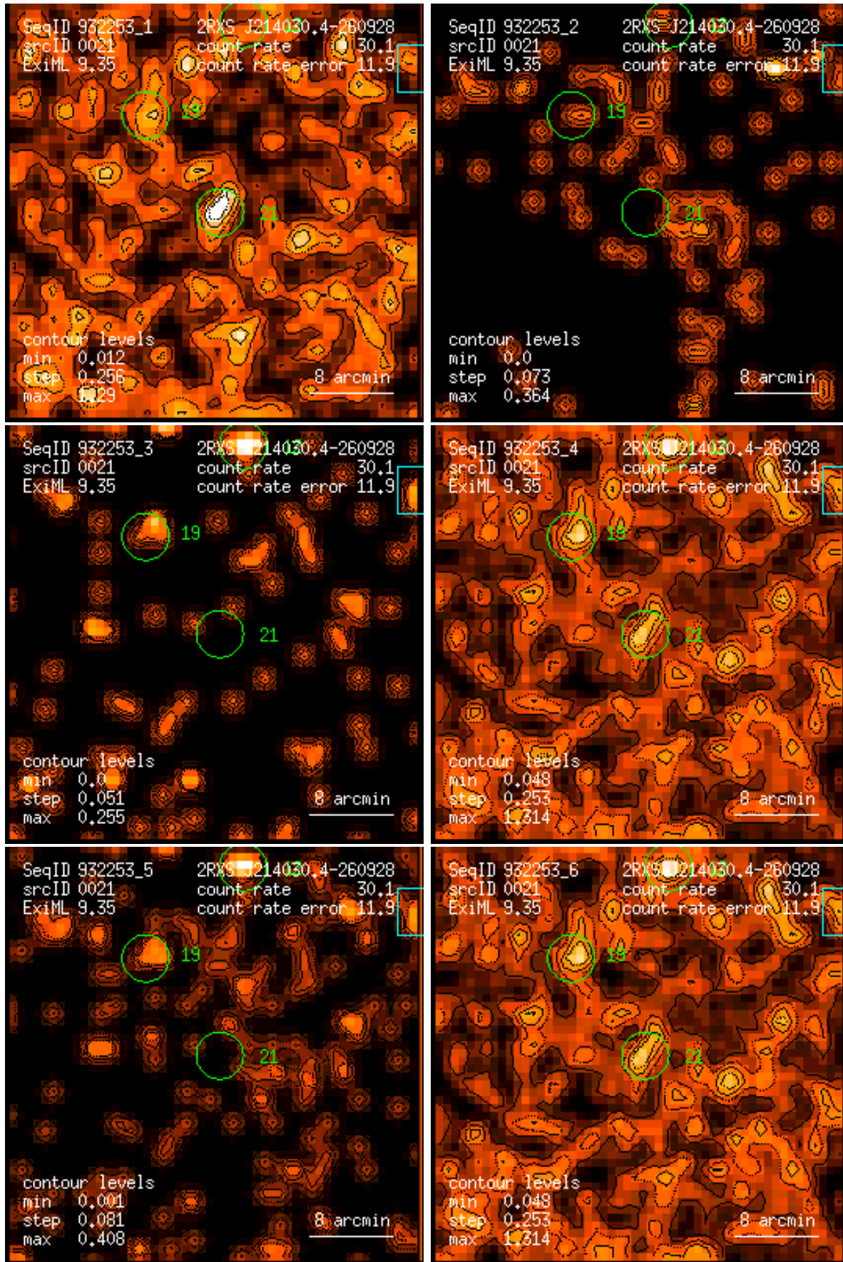
Figure 21: RASS 932253: detection 0021: band rate images, Gaussian filter: (1) PSPC channels 11 – 41, (2) 52 – 90, (3) 91 – 201, (4) 11 – 235, (5) 52 – 201, (6) 11 – 201. Broad band rates in counts/ks. Band rate contour levels in counts/ks/arcmin 2 .
