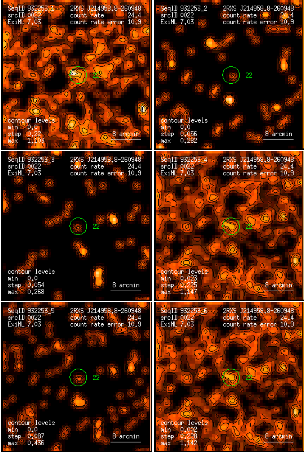
Figure 22: RASS 932253: detection 0022: band rate images, Gaussian filter: (1) PSPC channels 11 – 41, (2) 52 – 90, (3) 91 – 201, (4) 11 – 235, (5) 52 – 201, (6) 11 – 201. Broad band rates in counts/ks. Band rate contour levels in counts/ks/arcmin 2 .
