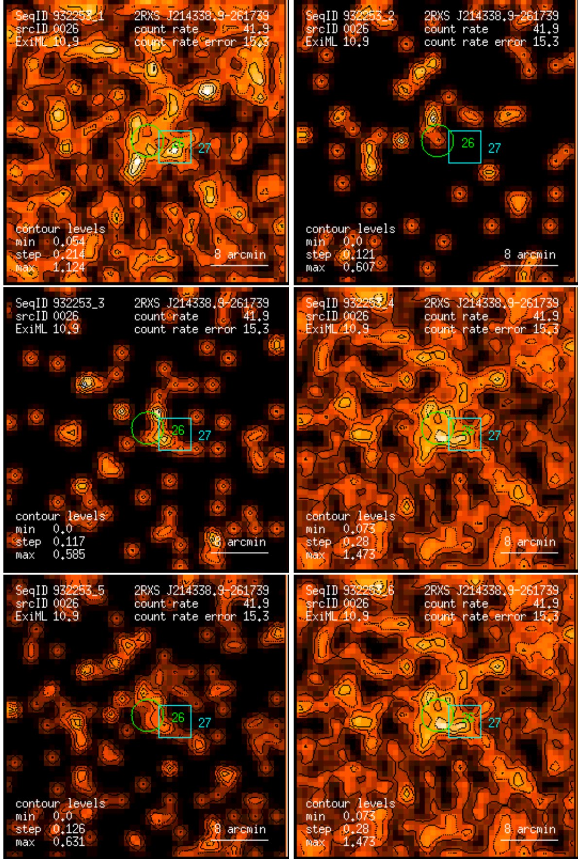
Figure 26: RASS 932253: detection 0026: band rate images, Gaussian filter: (1) PSPC channels 11 – 41, (2) 52 – 90, (3) 91 – 201, (4) 11 – 235, (5) 52 – 201, (6) 11 – 201. Broad band rates in counts/ks. Band rate contour levels in counts/ks/arcmin 2 .
