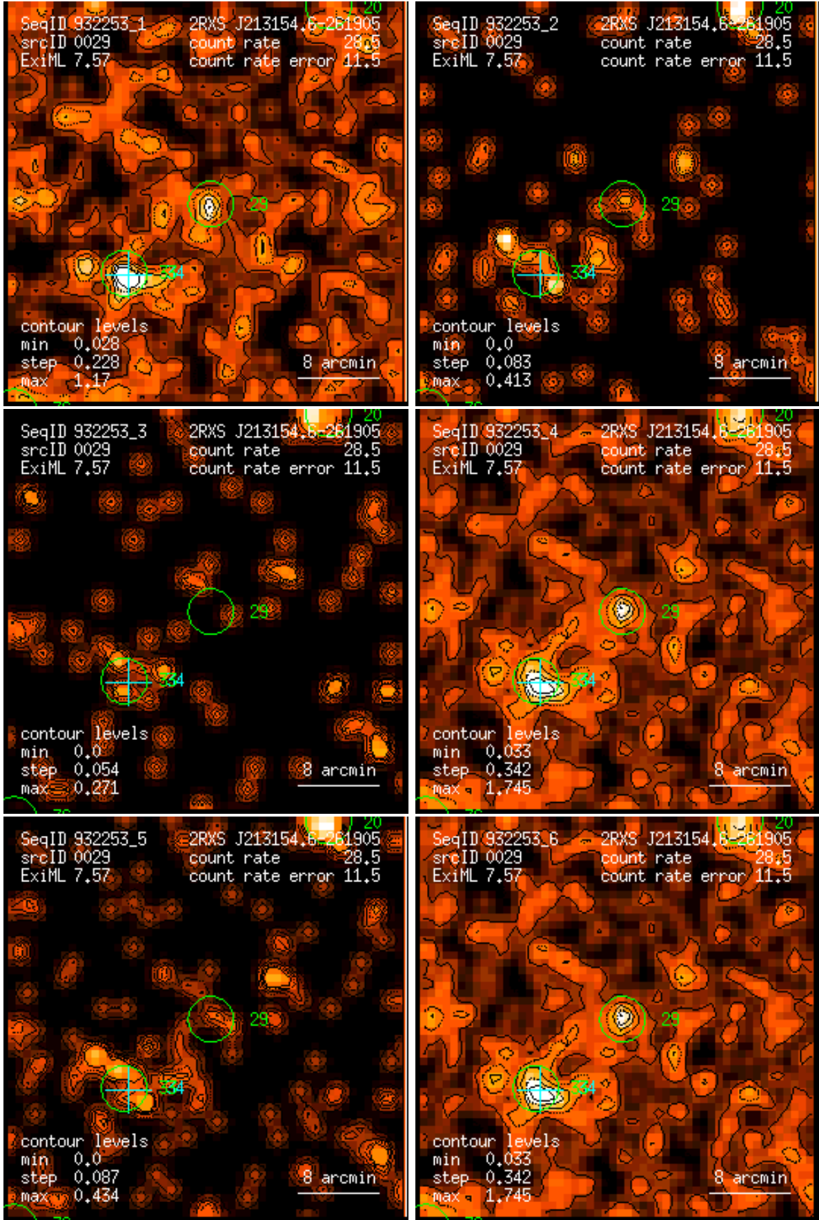
Figure 29: RASS 932253: detection 0029: band rate images, Gaussian filter: (1) PSPC channels 11 – 41, (2) 52 – 90, (3) 91 – 201, (4) 11 – 235, (5) 52 – 201, (6) 11 – 201. Broad band rates in counts/ks. Band rate contour levels in counts/ks/arcmin 2 .
