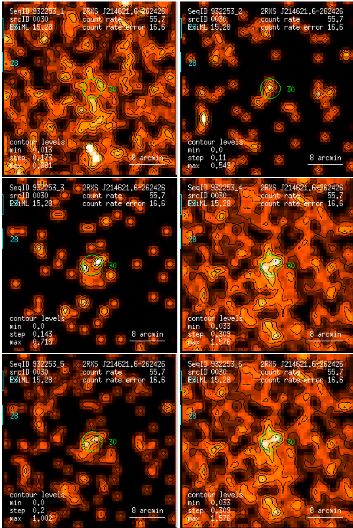
Figure 30: RASS 932253: detection 0030: band rate images, Gaussian filter: (1) PSPC channels 11 – 41, (2) 52 – 90, (3) 91 – 201, (4) 11 – 235, (5) 52 – 201, (6) 11 – 201. Broad band rates in counts/ks. Band rate contour levels in counts/ks/arcmin 2 .
