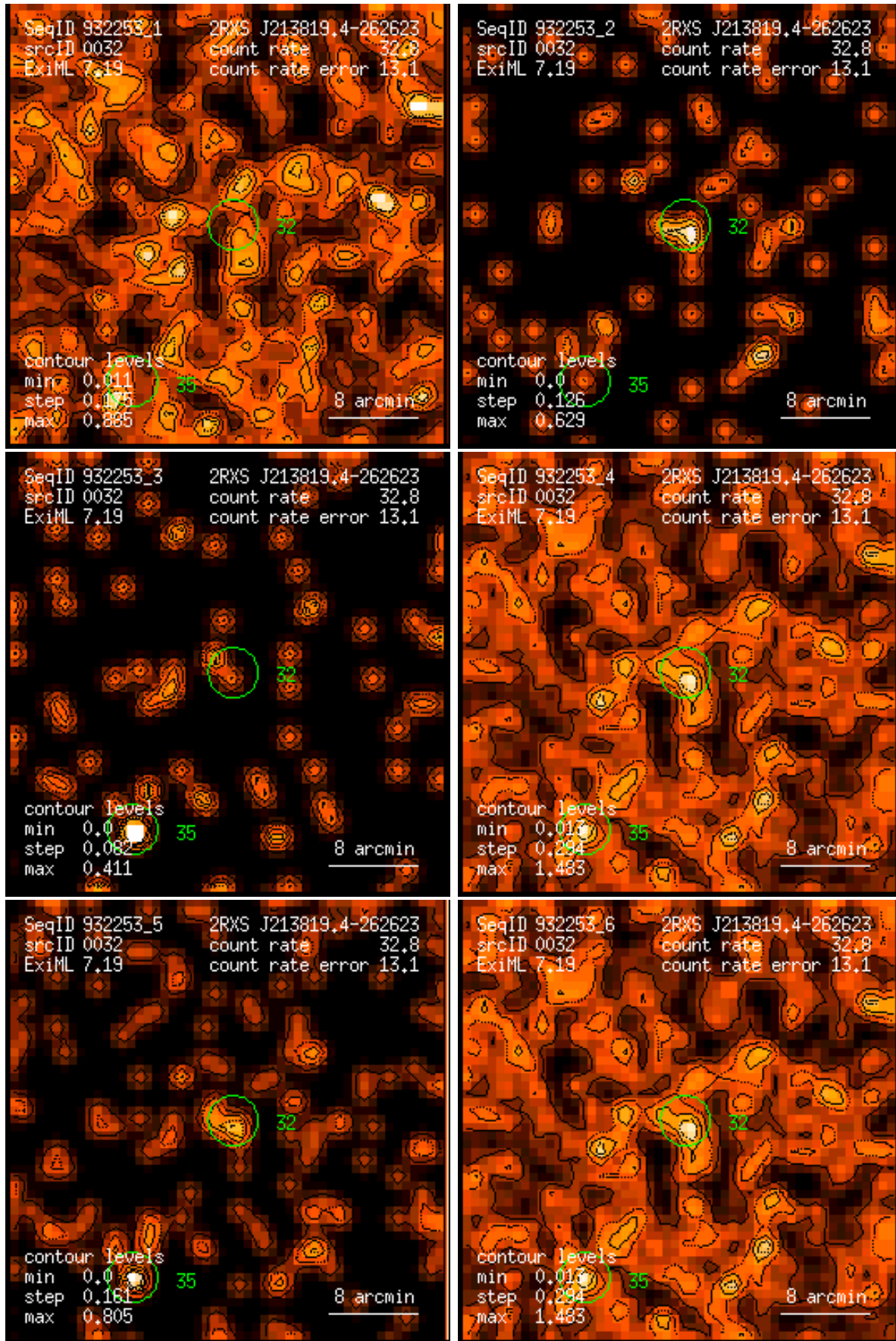
Figure 32: RASS 932253: detection 0032: band rate images, Gaussian filter: (1) PSPC channels 11 – 41, (2) 52 – 90, (3) 91 – 201, (4) 11 – 235, (5) 52 – 201, (6) 11 – 201. Broad band rates in counts/ks. Band rate contour levels in counts/ks/arcmin 2 .
