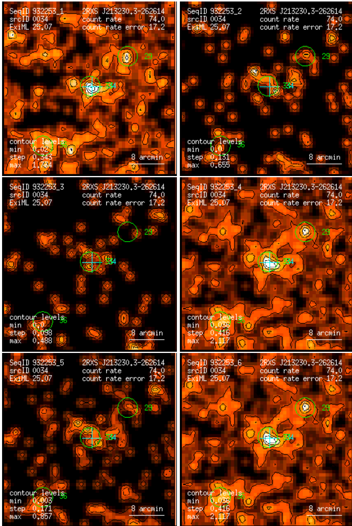
Figure 34: RASS 932253: detection 0034: band rate images, Gaussian filter: (1) PSPC channels 11 – 41, (2) 52 – 90, (3) 91 – 201, (4) 11 – 235, (5) 52 – 201, (6) 11 – 201. Broad band rates in counts/ks. Band rate contour levels in counts/ks/arcmin 2 .
