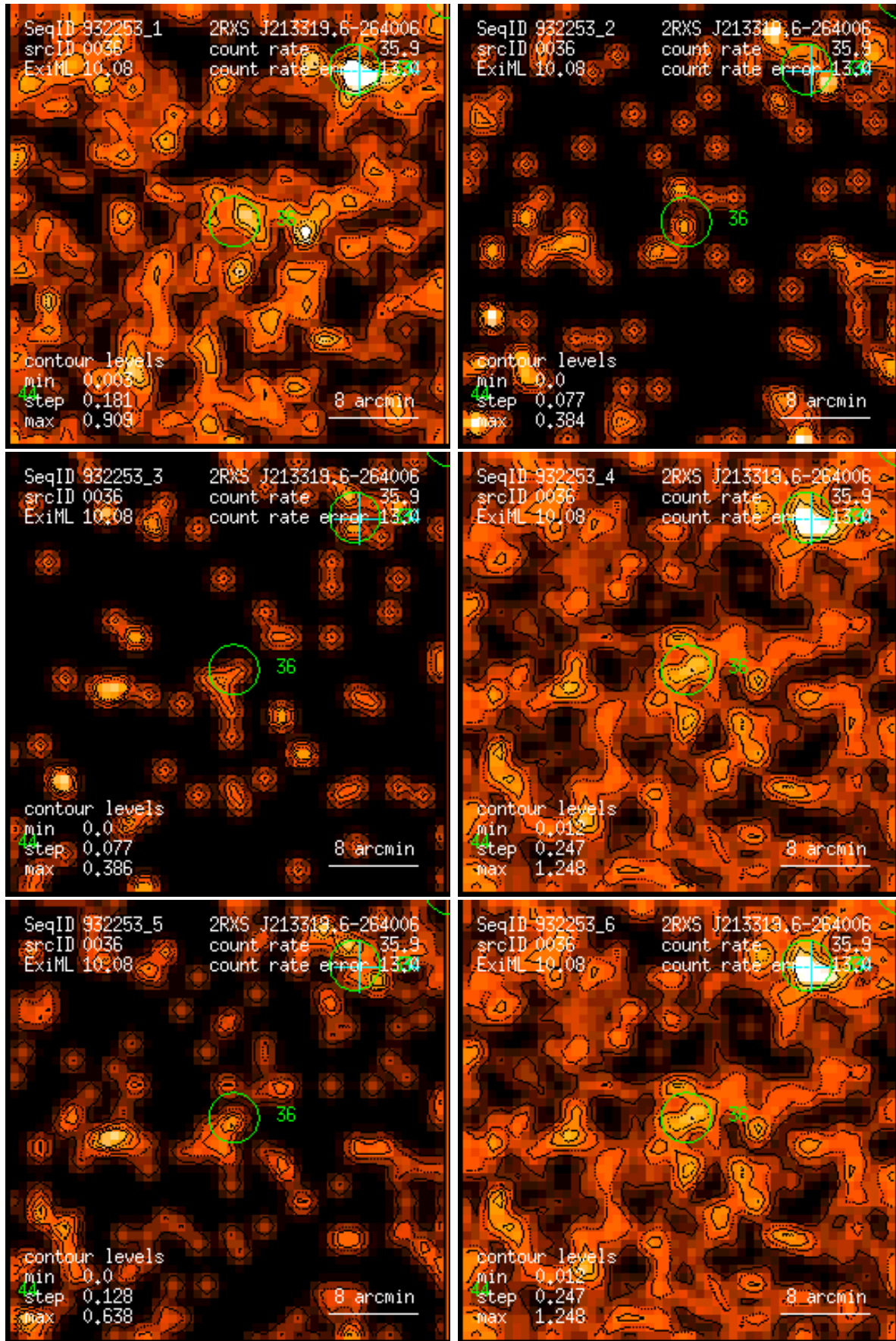
Figure 36: RASS 932253: detection 0036: band rate images, Gaussian filter: (1) PSPC channels 11 – 41, (2) 52 – 90, (3) 91 – 201, (4) 11 – 235, (5) 52 – 201, (6) 11 – 201. Broad band rates in counts/ks. Band rate contour levels in counts/ks/arcmin 2 .
