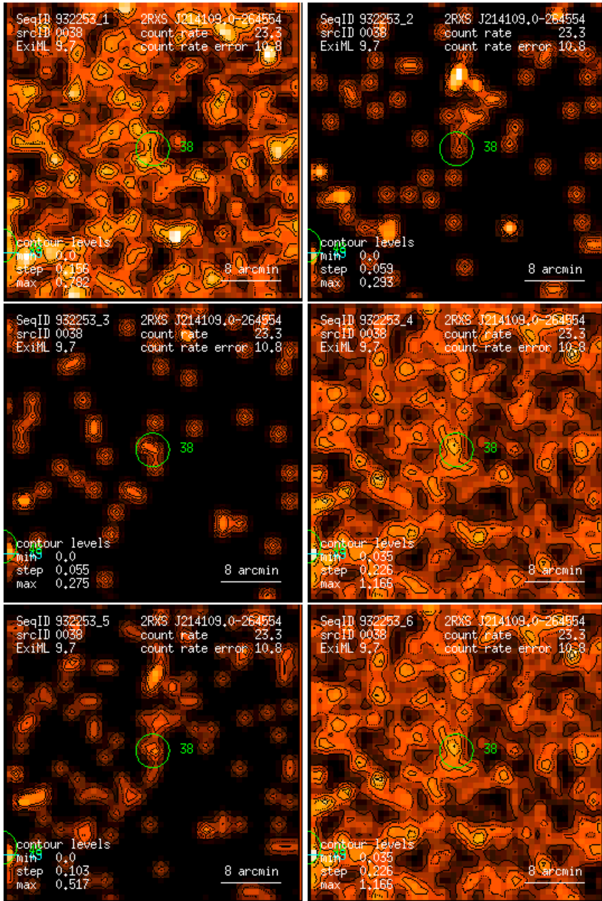
Figure 38: RASS 932253: detection 0038: band rate images, Gaussian filter: (1) PSPC channels 11 – 41, (2) 52 – 90, (3) 91 – 201, (4) 11 – 235, (5) 52 – 201, (6) 11 – 201. Broad band rates in counts/ks. Band rate contour levels in counts/ks/arcmin 2 .
