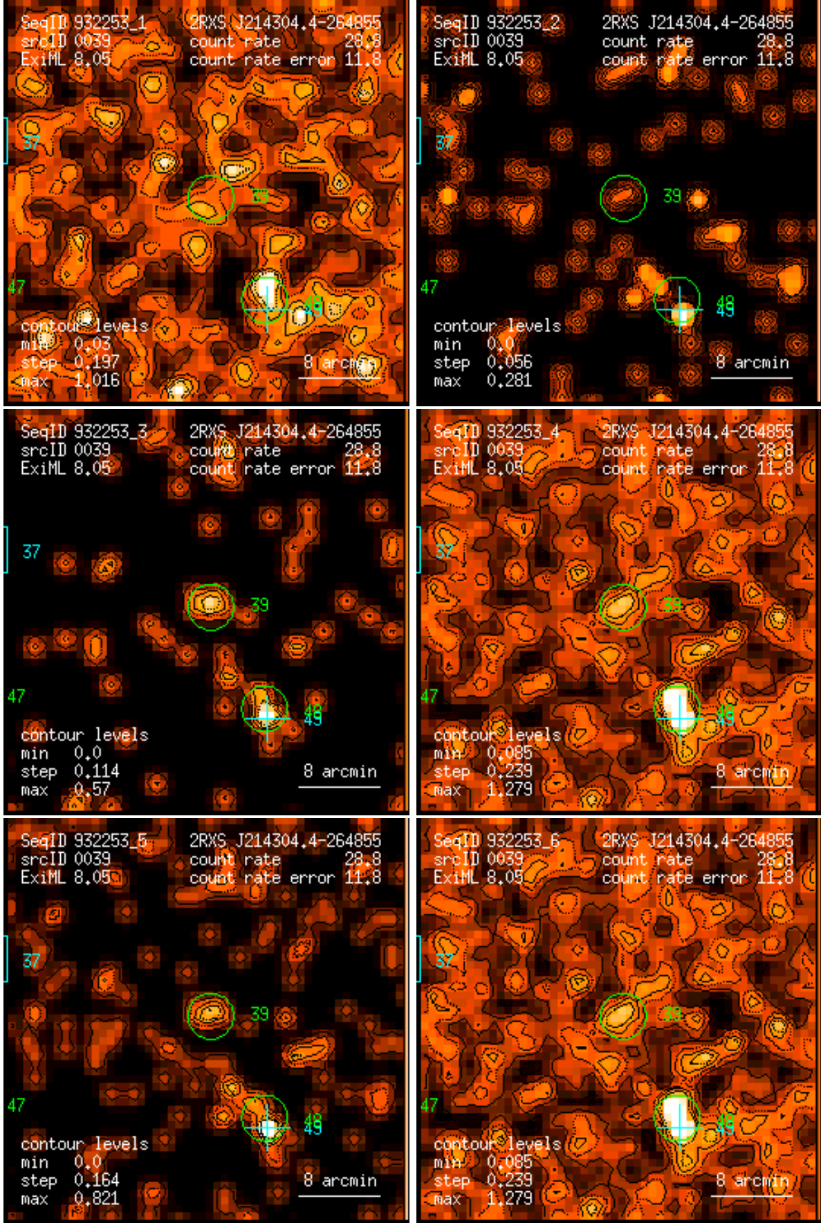
Figure 39: RASS 932253: detection 0039: band rate images, Gaussian filter: (1) PSPC channels 11 – 41, (2) 52 – 90, (3) 91 – 201, (4) 11 – 235, (5) 52 – 201, (6) 11 – 201. Broad band rates in counts/ks. Band rate contour levels in counts/ks/arcmin 2 .
