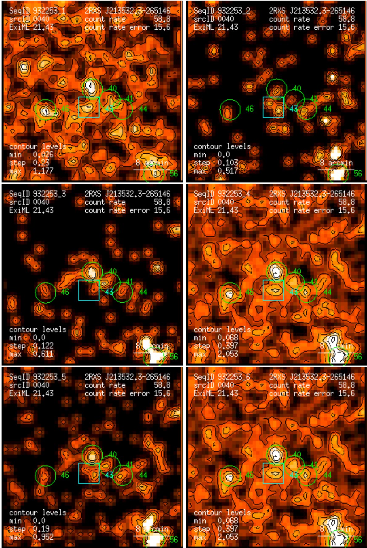
Figure 40: RASS 932253: detection 0040: band rate images, Gaussian filter: (1) PSPC channels 11 – 41, (2) 52 – 90, (3) 91 – 201, (4) 11 – 235, (5) 52 – 201, (6) 11 – 201. Broad band rates in counts/ks. Band rate contour levels in counts/ks/arcmin 2 .
