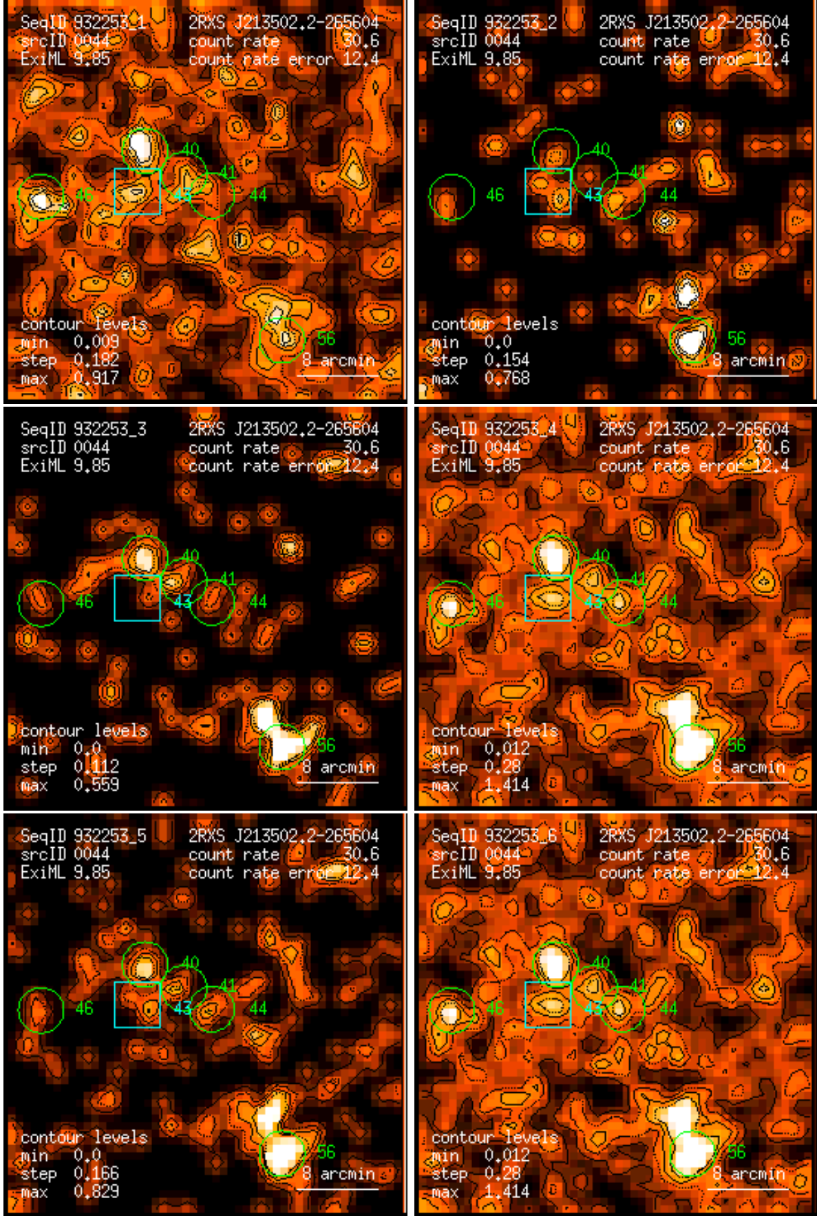
Figure 44: RASS 932253: detection 0044: band rate images, Gaussian filter: (1) PSPC channels 11 – 41, (2) 52 – 90, (3) 91 – 201, (4) 11 – 235, (5) 52 – 201, (6) 11 – 201. Broad band rates in counts/ks. Band rate contour levels in counts/ks/arcmin 2 .
