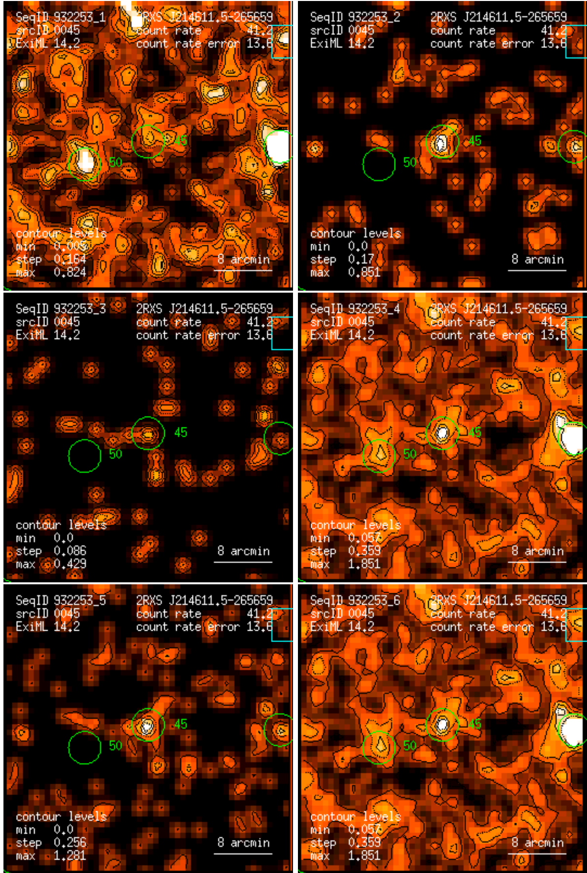
Figure 45: RASS 932253: detection 0045: band rate images, Gaussian filter: (1) PSPC channels 11 – 41, (2) 52 – 90, (3) 91 – 201, (4) 11 – 235, (5) 52 – 201, (6) 11 – 201. Broad band rates in counts/ks. Band rate contour levels in counts/ks/arcmin 2 .
