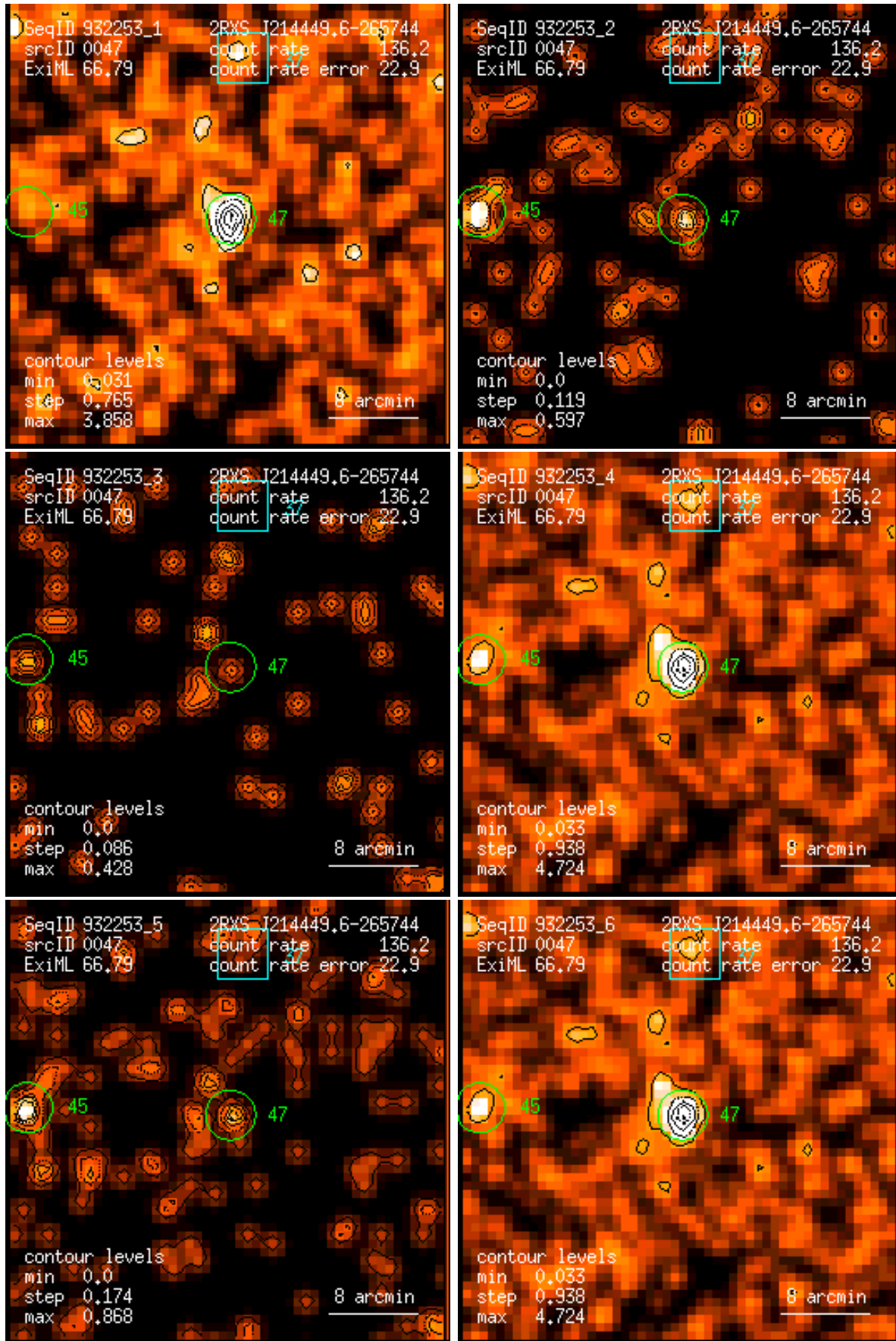
Figure 47: RASS 932253: detection 0047: band rate images, Gaussian filter: (1) PSPC channels 11 – 41, (2) 52 – 90, (3) 91 – 201, (4) 11 – 235, (5) 52 – 201, (6) 11 – 201. Broad band rates in counts/ks. Band rate contour levels in counts/ks/arcmin 2 .
