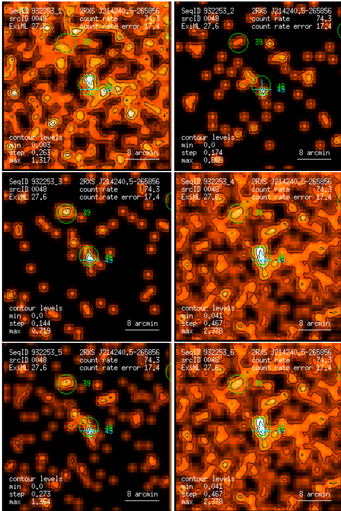
Figure 48: RASS 932253: detection 0048: band rate images, Gaussian filter: (1) PSPC channels 11 – 41, (2) 52 – 90, (3) 91 – 201, (4) 11 – 235, (5) 52 – 201, (6) 11 – 201. Broad band rates in counts/ks. Band rate contour levels in counts/ks/arcmin 2 .
