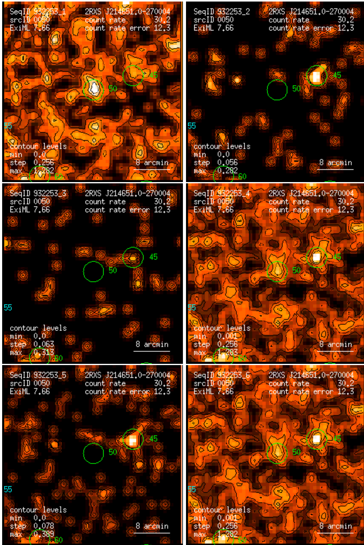
Figure 50: RASS 932253: detection 0050: band rate images, Gaussian filter: (1) PSPC channels 11 – 41, (2) 52 – 90, (3) 91 – 201, (4) 11 – 235, (5) 52 – 201, (6) 11 – 201. Broad band rates in counts/ks. Band rate contour levels in counts/ks/arcmin 2 .
