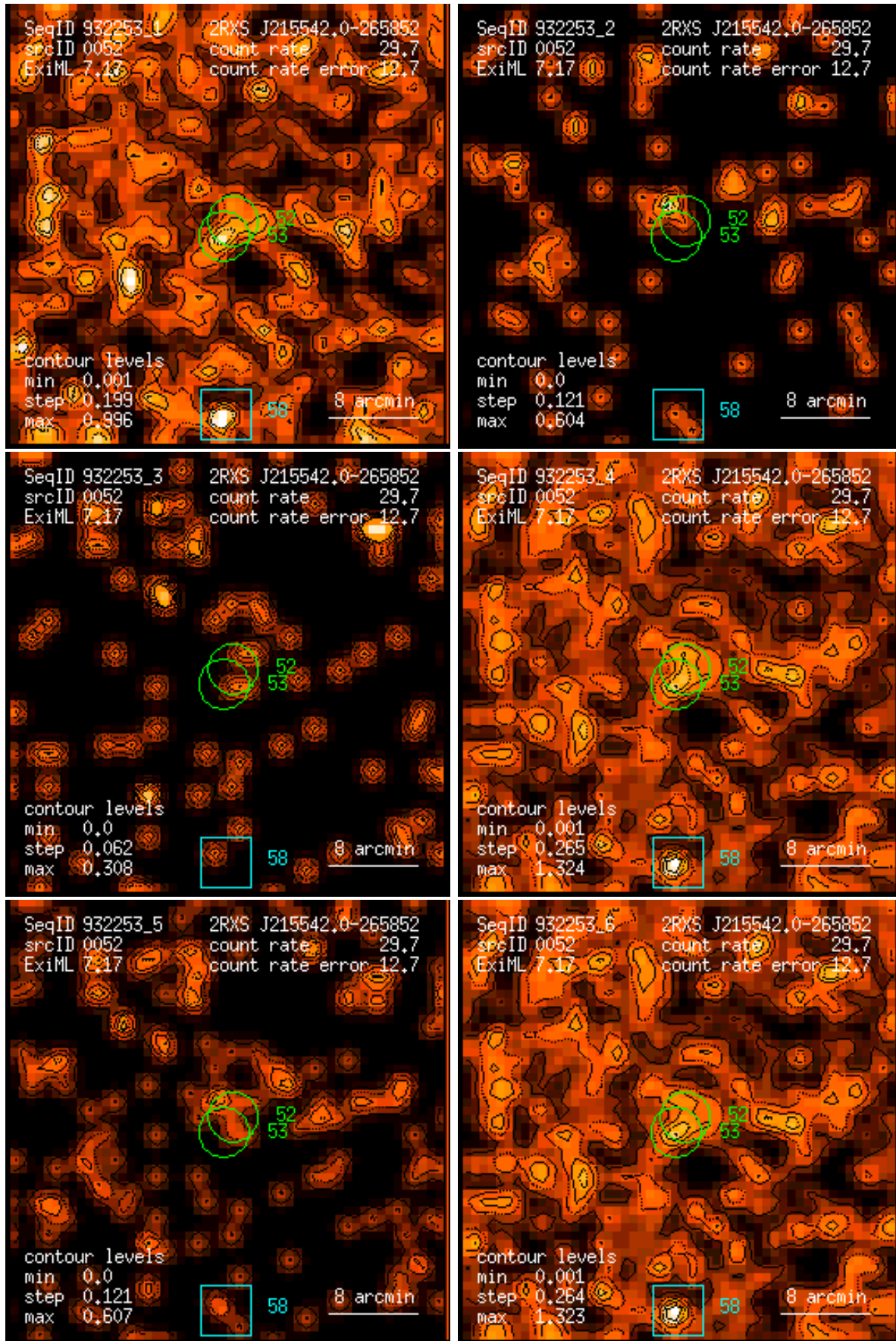
Figure 52: RASS 932253: detection 0052: band rate images, Gaussian filter: (1) PSPC channels 11 – 41, (2) 52 – 90, (3) 91 – 201, (4) 11 – 235, (5) 52 – 201, (6) 11 – 201. Broad band rates in counts/ks. Band rate contour levels in counts/ks/arcmin 2 .
