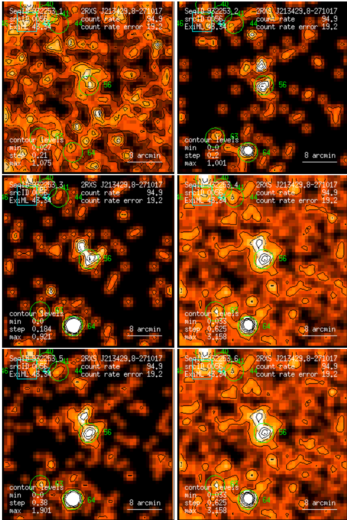
Figure 56: RASS 932253: detection 0056: band rate images, Gaussian filter: (1) PSPC channels 11 – 41, (2) 52 – 90, (3) 91 – 201, (4) 11 – 235, (5) 52 – 201, (6) 11 – 201. Broad band rates in counts/ks. Band rate contour levels in counts/ks/arcmin 2 .
